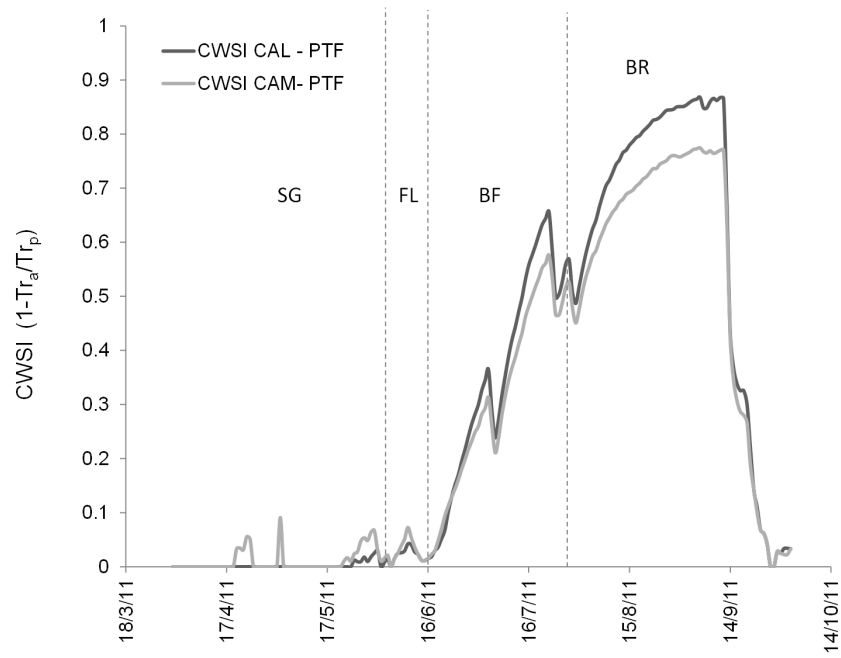
Fig. 3. CWSI obtained with hydraulic properties estimated (PTF)
