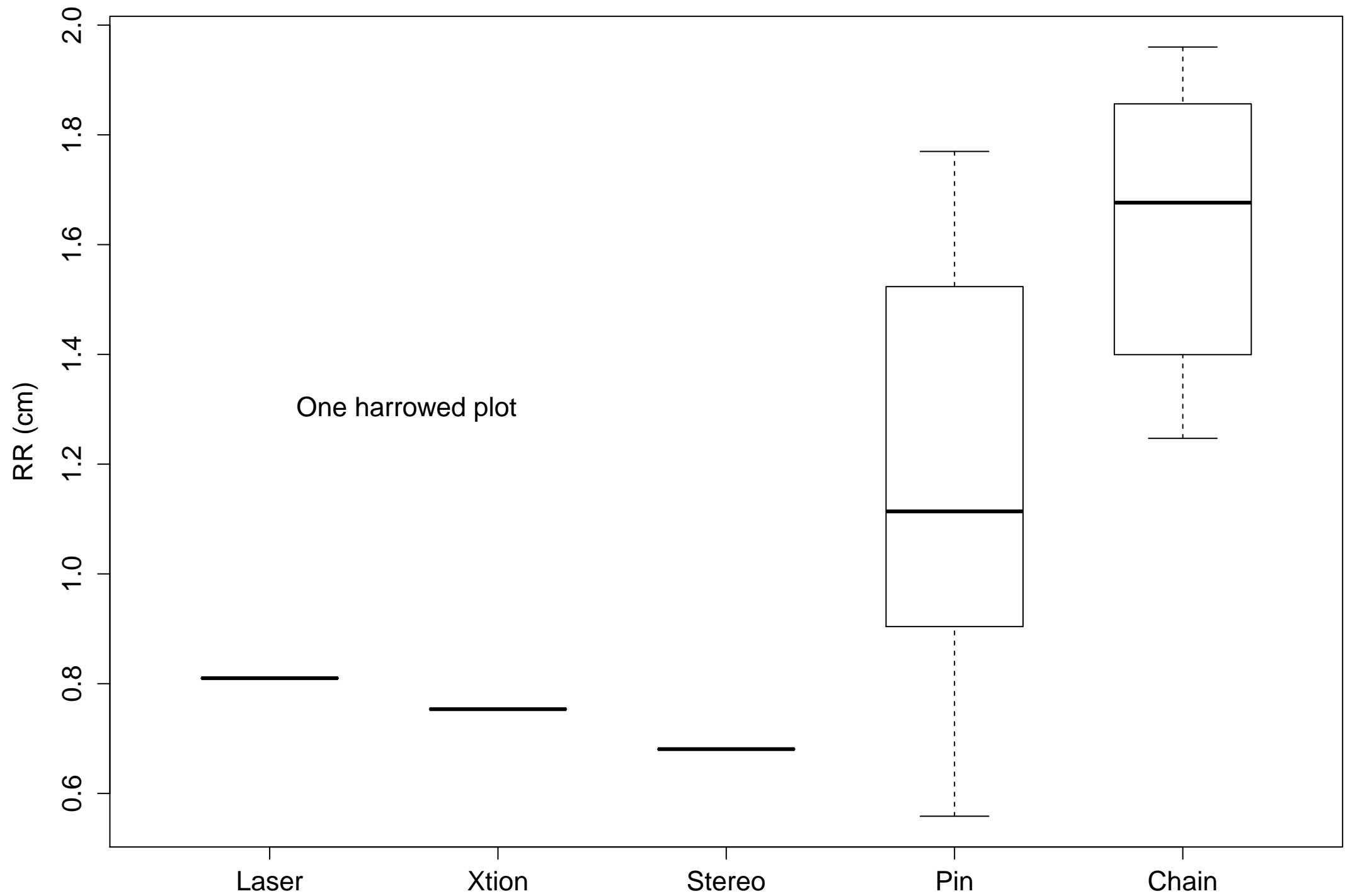
Measured roughness on harrowed soil surface
