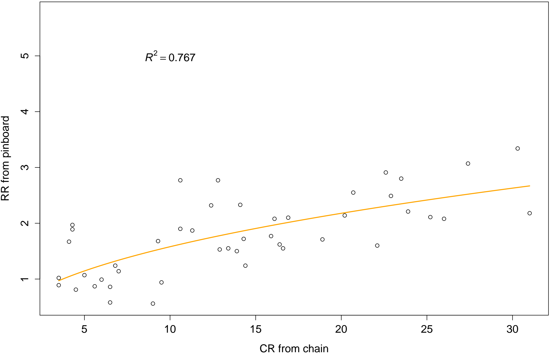
Regression between CR and RR, y=0.543x^{0.464}
