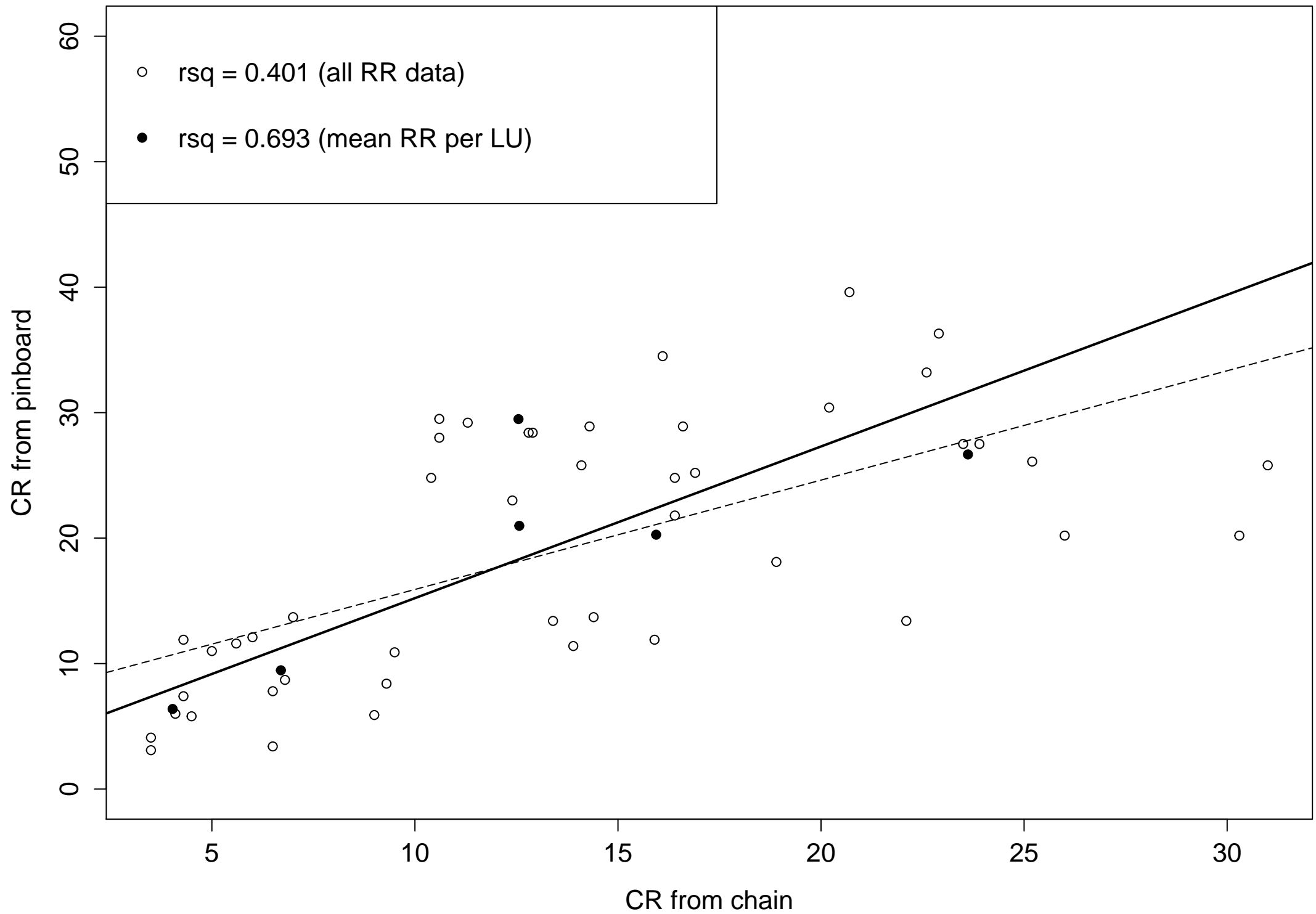
Scatterplot of the CR-index measured with the roller chain and calculated from the pinboard
