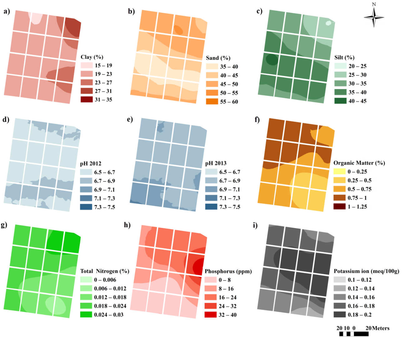
456 Figure 2. Maps of spatial distribution of some soil components in the vineyard site: a) Clay; b) Sand; c) Silt; d) pH of 457 2012 growing season; e) pH of 2013 growing season; f) Organic matter; g) Total Nitrogen; h) Assimilable phosphorus; i) 458 Potassium ion (K).
