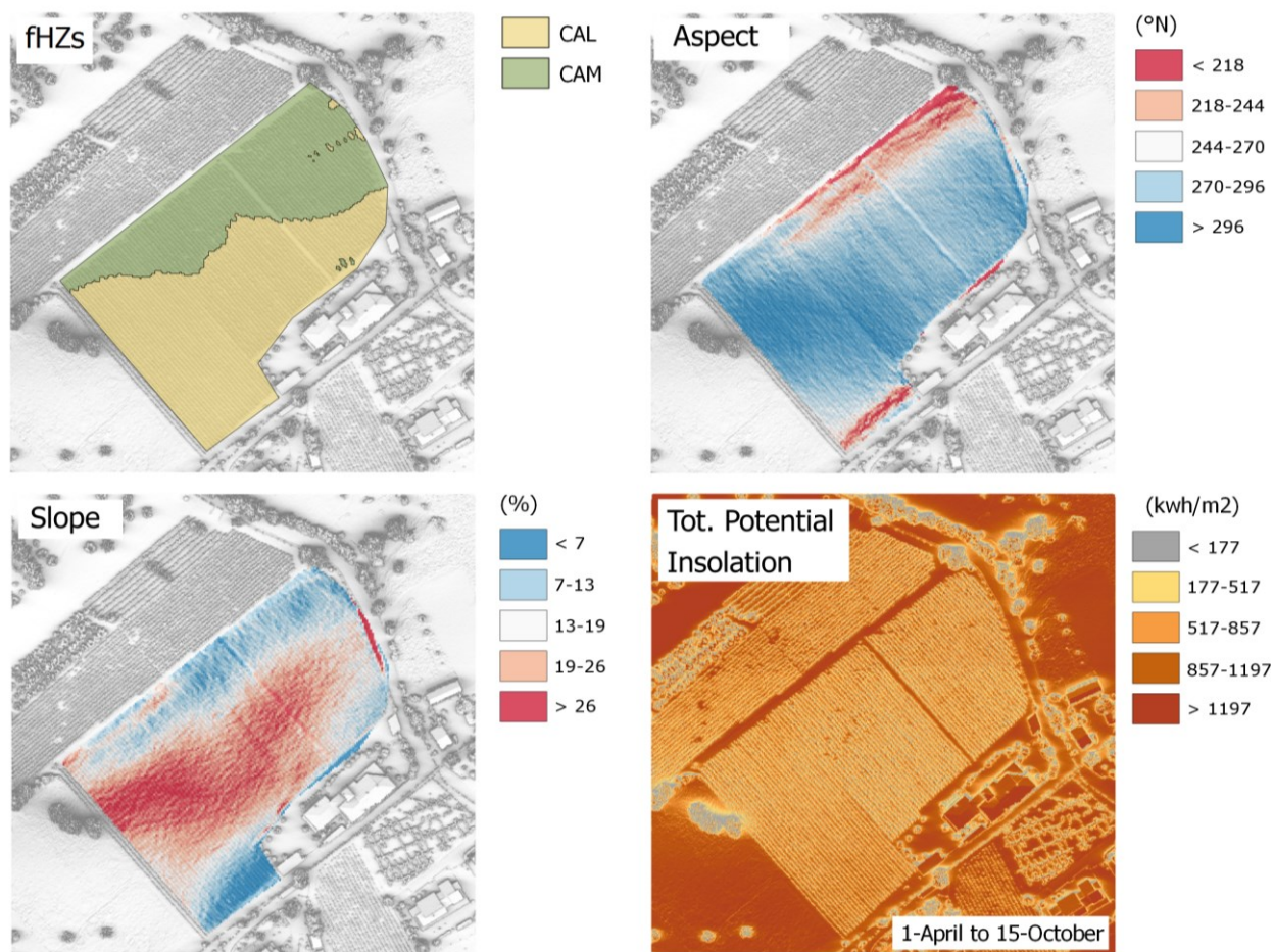
Fig. 6. The functional homogenous zones (fHZs) identified in the study area and the three maps derived from DSM and DTM analysis in a G.I.S environment: Aspect, Slope and Total Potential Insolation.
