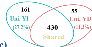
ASVs used for network contribution
