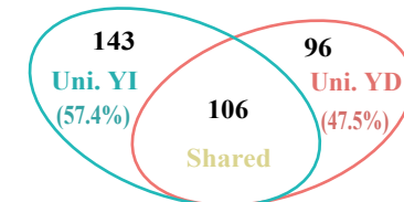
Nodes in network modules
