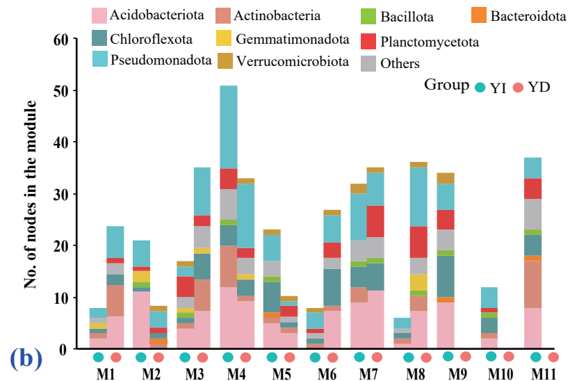
ASVs used for network contribution
