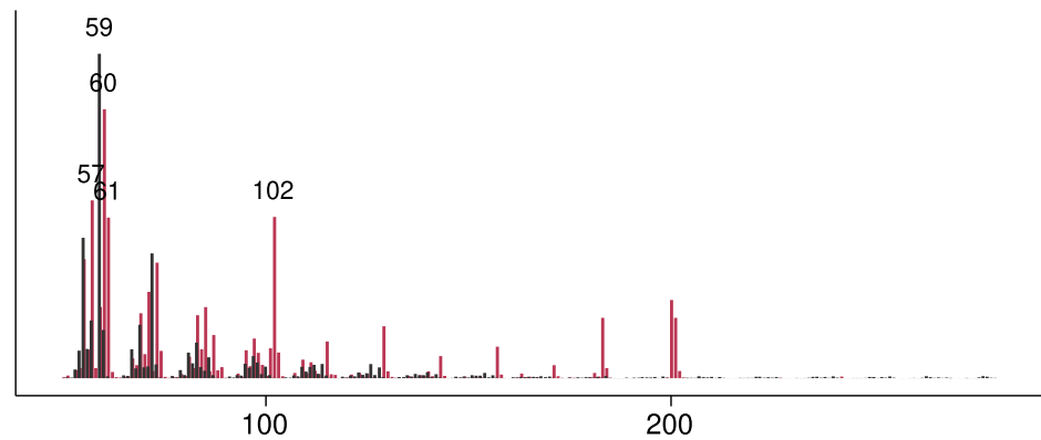
Propyl dodecanoate
