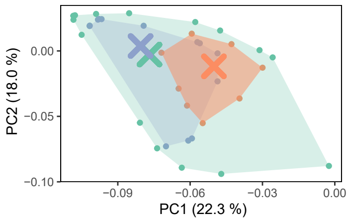
Data set hulls and centroids (mean)
