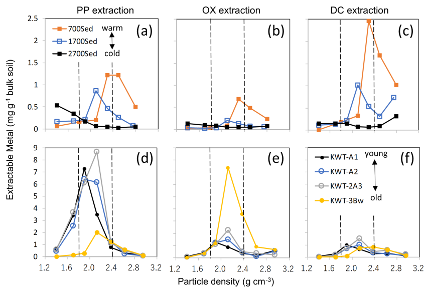
Figure A8. The distribution of the extractable metal phases ( Al + 0.5Fe ) along the particle density gradient for two soil series. The upper three plots show PP- (a), OX- (b), and DC-extractable metals (c) for three A horizon soils under tropical forest along an elevation gradient from a weathered soil under warm climate at 700 m (sample ID: C5), moderately weathered soil at 1700 m (C6), and much less weathered soil at 2700 m (C7). The lower panels (d, e, f) showed surface and buried horizons of a non-allophanic Andisol profile (sample ID: N1–N4) that received multiple tephra deposits. Shaded zones show the meso-density range.
