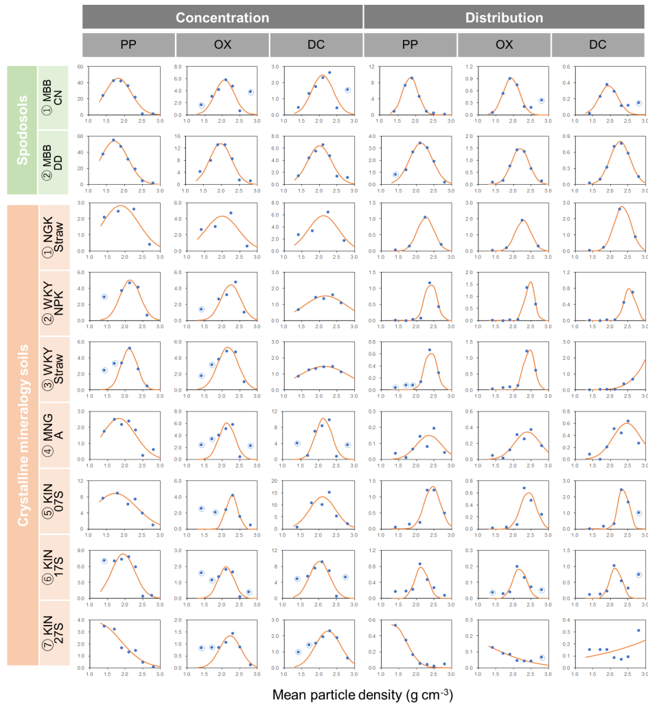
Figure A1. Extractable metal ( \text{Al} + 0.5 \text{Fe} ) against mean particle density for each soil sample. The metal concentrations ( \text{mg g}^{-1} fraction) from pyrophosphate (PP), acid oxalate (OX), and dithionite–citrate (DC) extractions are shown in the left three panels. The distributions of PP, OX, and DC-extractable metal phases ( \text{mg g}^{-1} whole soil) are in the right three panels. Normal distribution curve fit is shown as line. The data points circled in blue were omitted from the fitting.
