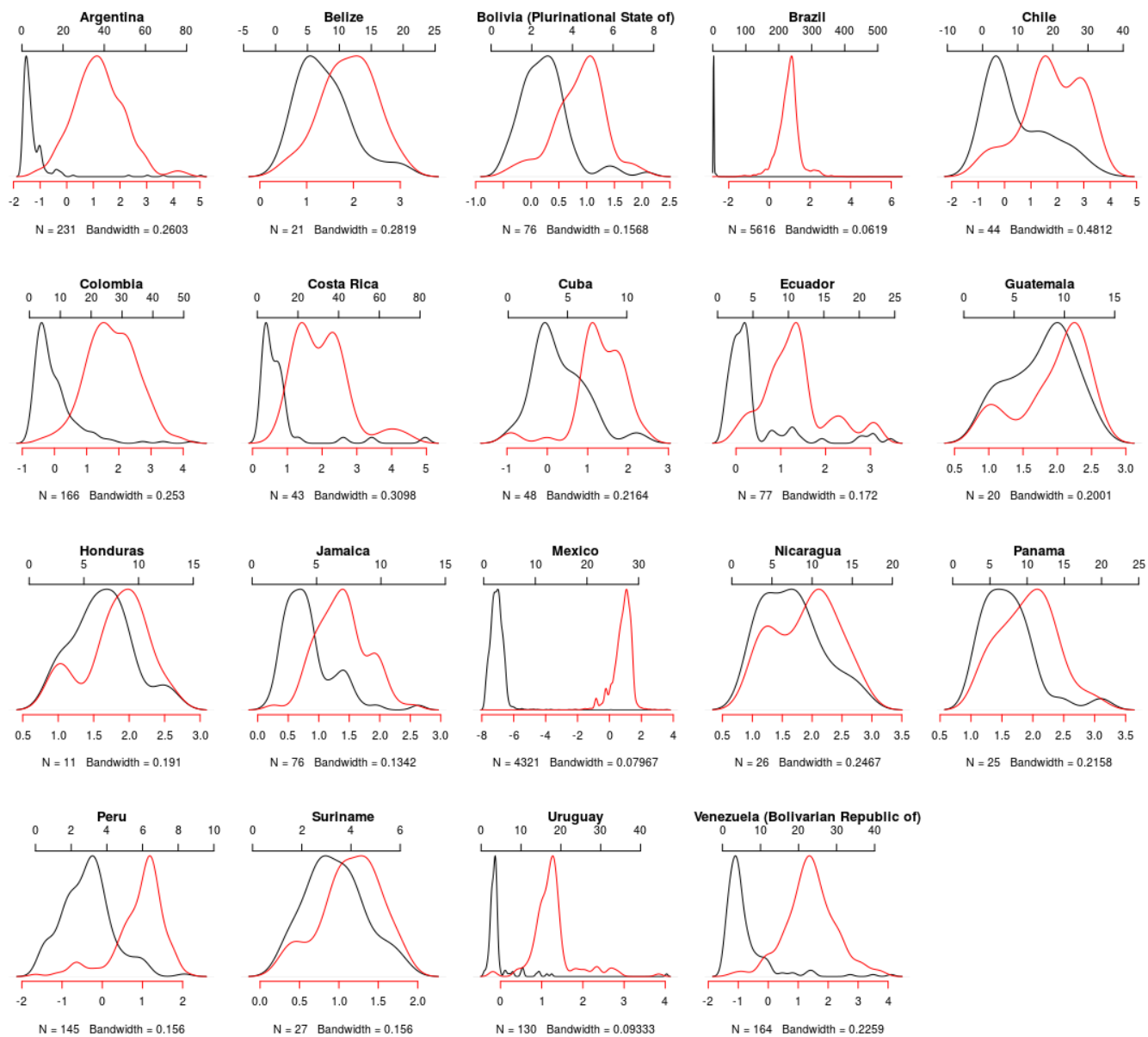
Figure S1. Probability distribution functions for the estimated SOC values (in kg.m 2 ) before (black lines) and after (red lines) the log transformation across the 19 analyzed countries.
