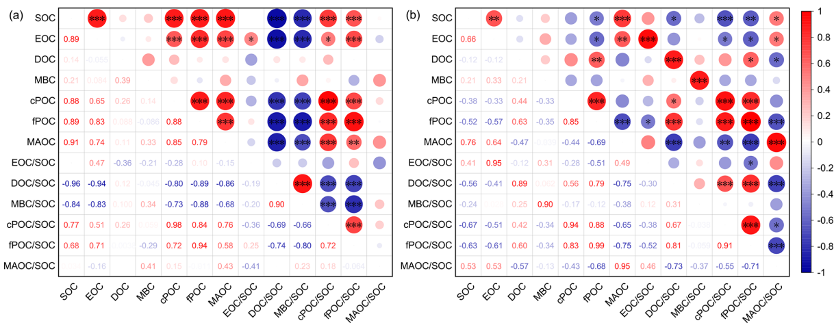
Figure 4. Pearson correlations among soil organic carbon (SOC) fractions and their relative proportions in greenhouses for (a) loam and (b) sandy loam. Note: SOC fractions represent concentrations ( \text{g kg}^{-1} ), include total SOC, easily oxidizable organic carbon (EOC), dissolved organic carbon (DOC), microbial biomass carbon (MBC), coarse particulate organic carbon (cPOC), fine particulate organic carbon (fPOC), and mineral-associated organic carbon (MAOC). Their relative proportions to SOC include EOC/SOC, DOC/SOC, MBC/SOC, cPOC/SOC, fPOC/SOC, and MAOC/SOC. * Correlation was significant at P \leq 0.05 ; ** Correlation was significant at P \leq 0.01 ; *** Correlation was significant at P \leq 0.001 .
