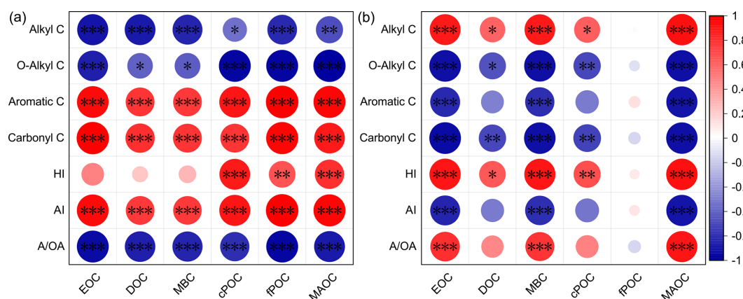
Figure 6. Pearson correlations between soil organic carbon (SOC) fractions based on their concentrations ( \text{g kg}^{-1} ) and SOC chemical structure and stability indices in greenhouses (a) loam and (b) sandy loam. Note: SOC fractions include total SOC, easily oxidizable organic carbon (EOC), dissolved organic carbon (DOC), microbial biomass carbon (MBC), coarse particulate organic carbon (cPOC), fine particulate organic carbon (fPOC), and mineral-associated organic carbon (MAOC). SOC stability indices include aromaticity index (AI), hydrophobicity index (HI), and the ratio of alkyl C to O-alkyl C (A/OA). * Correlation was significant at P \leq 0.05 ; ** Correlation was significant at P \leq 0.01 ; *** Correlation was significant at P \leq 0.001 .
