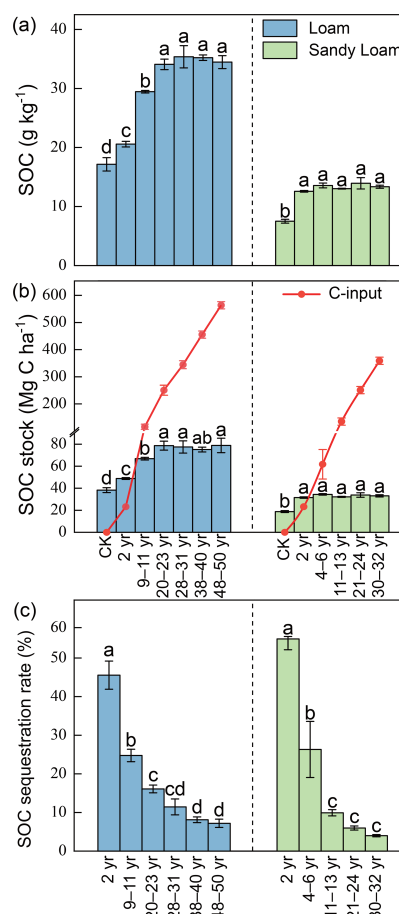
Figure 1. Changes in (a) soil organic carbon (SOC), (b) manure-derived carbon input and SOC stock, and (c) SOC sequestration rate following manure application over various years in greenhouses. Bars represent the standard errors. Within each soil texture, bars with different lowercase letters indicate significant differences among years of manure application ( P < 0.05 ).
