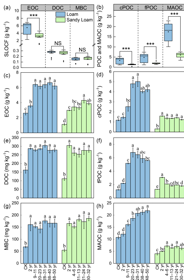
Figure 2. Content and variations of (a) soil labile organic carbon fractions (SLOCF), (b) particulate organic carbon (POC), and mineral-associated organic carbon (MAOC) with data pooled across all years of manure application in greenhouse (loam and sandy loam); and dynamic changes in (c) easily oxidizable organic carbon (EOC), (e) dissolved organic carbon (DOC), (g) microbial biomass carbon (MBC), (d) coarse particulate organic carbon (cPOC), (f) fine particulate organic carbon (fPOC), and (h) mineral-associated organic carbon (MAOC) across different years of manure application in greenhouse soils. Bars represent the standard errors. Within each soil texture, bars with different lowercase letters indicate significant differences among years of manure application ( P < 0.05 ).
