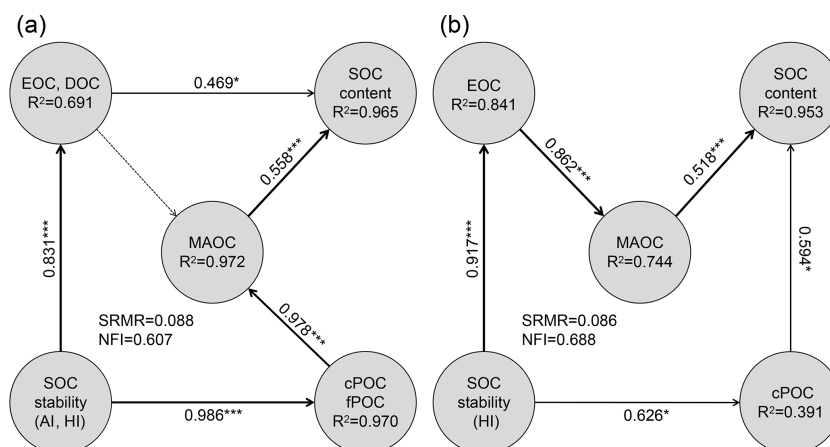
Figure 7. Partial least squares structural equation models (PLS-SEM) illustrating the pathways through which soil organic carbon (SOC) chemical stability indices influence SOC fractions and SOC content in greenhouse soils: (a) loam; (b) sandy loam. Numbers on arrows denote path coefficients, while numbers adjacent to arrows represent weight contributions. Solid and dashed lines indicate significant and non-significant relationships, respectively. Note: SOC fractions include easily oxidizable organic carbon (EOC), dissolved organic carbon (DOC), coarse particulate organic carbon (cPOC), fine particulate organic carbon (fPOC), and mineral-associated organic carbon (MAOC). SOC chemical stability indices include aromaticity index (AI) and hydrophobicity index (HI).
