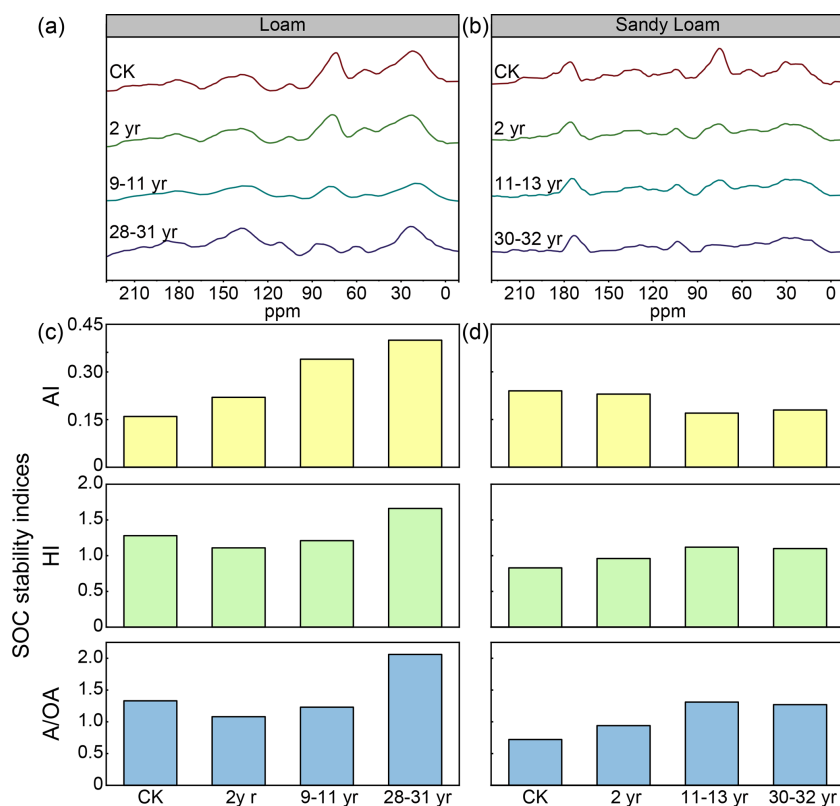
Figure 5. Solid-state CPMAS 13 C NMR spectroscopy of greenhouse soils under varying years of manure application in (a) loam and (b) sandy loam. Soil organic carbon (SOC) stability indicators during different manure application years in (c) loam and (d) sandy loam under greenhouse conditions. A/OA: the ratio of alkyl C to O-alkyl C; HI: hydrophobicity index; AI: aromaticity index.
