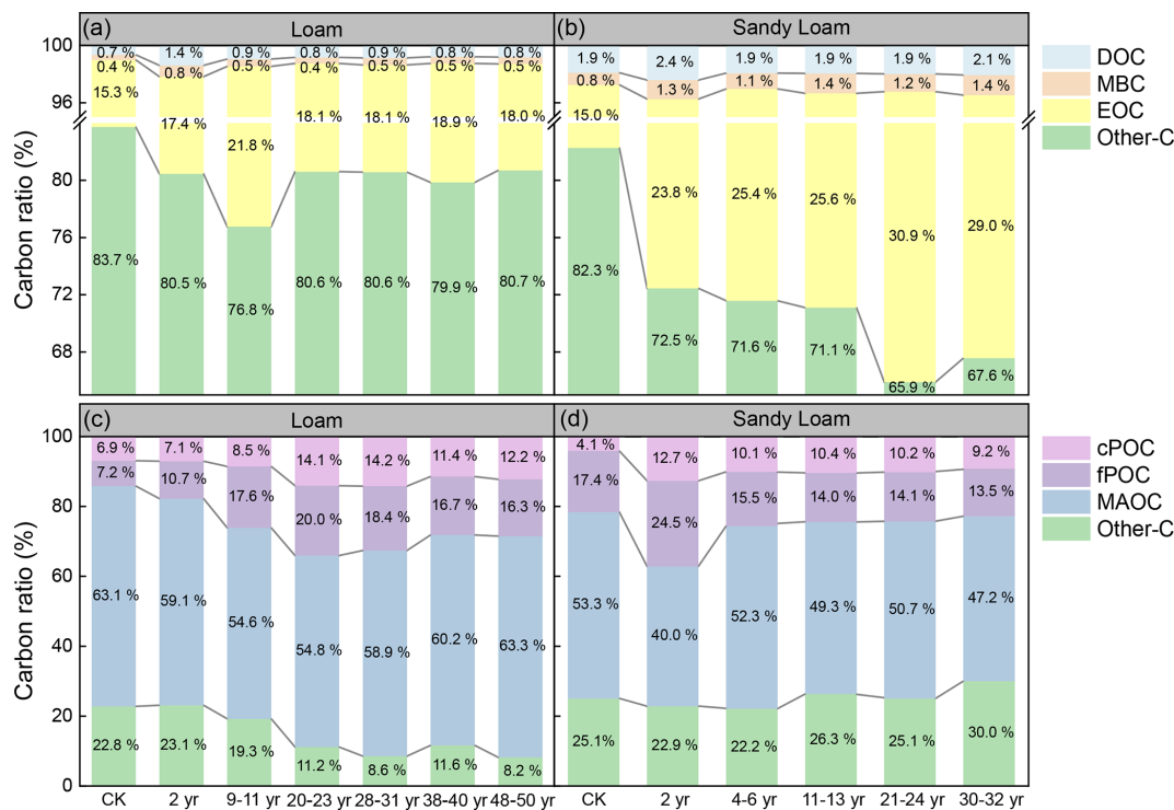
Figure 3. Proportions of soil labile organic carbon fractions (SLOCF: easily oxidizable organic carbon [EOC], microbial biomass carbon [MBC], and dissolved organic carbon [DOC]), particulate organic carbon (POC: coarse POC [cPOC] and fine POC [fPOC]), and mineral-associated organic carbon (MAOC) to soil organic carbon (SOC) in greenhouse soils under different manure application years in (a, c) loam and (b, d) sandy loam.
