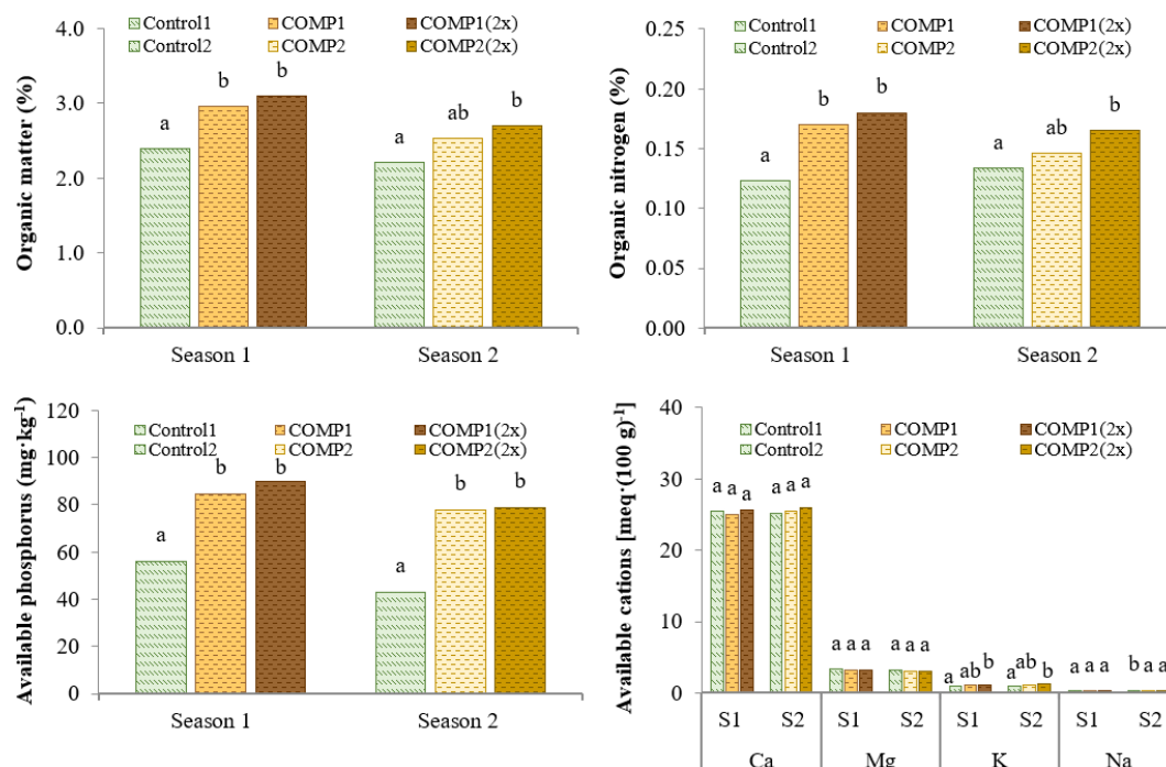
Figure 1. Concentration of organic matter, organic nitrogen, available phosphorus and cations of the soil from both seasons. COMP1: compost 1 (PR); COMP2 (RS): compost 2 (RS). Different letters indicate significant differences between treatments in each season according to Fisher's LSD test ( p < 0.05 ).
