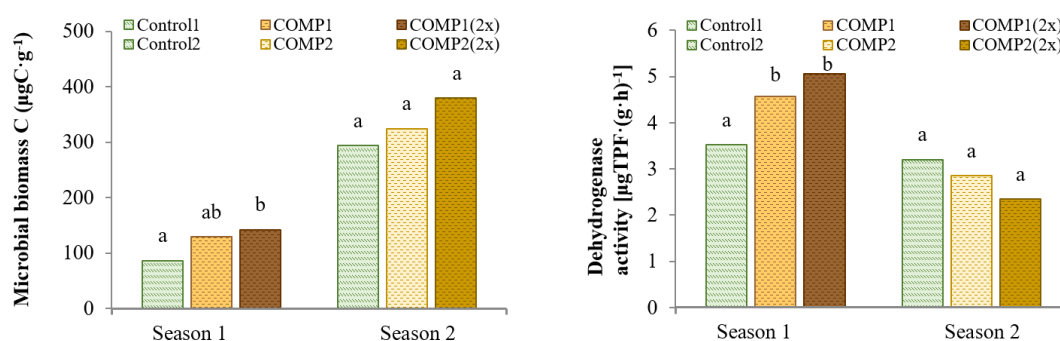
Figure 2. Soil biomass carbon and dehydrogenase activity from both seasons. COMP1: compost 1 (PR); COMP2 (RS): compost 2 (RS). Different letters indicate significant differences between treatments in each season according to Fisher's LSD test ( p < 0.05 ).
