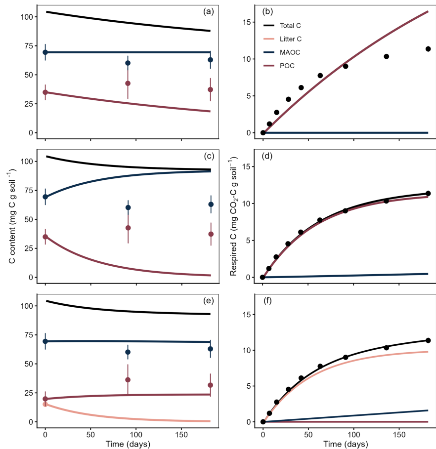
Figure 3. C content (a, c, e) and respired C (b, d, f) in each C pool and total in litter-addition treatments. In black, Total C; in dark blue, MAOC; in dark red, POC; in pink, Litter C. The lines represent the model estimations, while the points represent the observed data. (a, b) 2-pool models that best fitted C pools content. (c, d) 2-pool models that best fitted the respiration. (e, f) 3-pool model.
