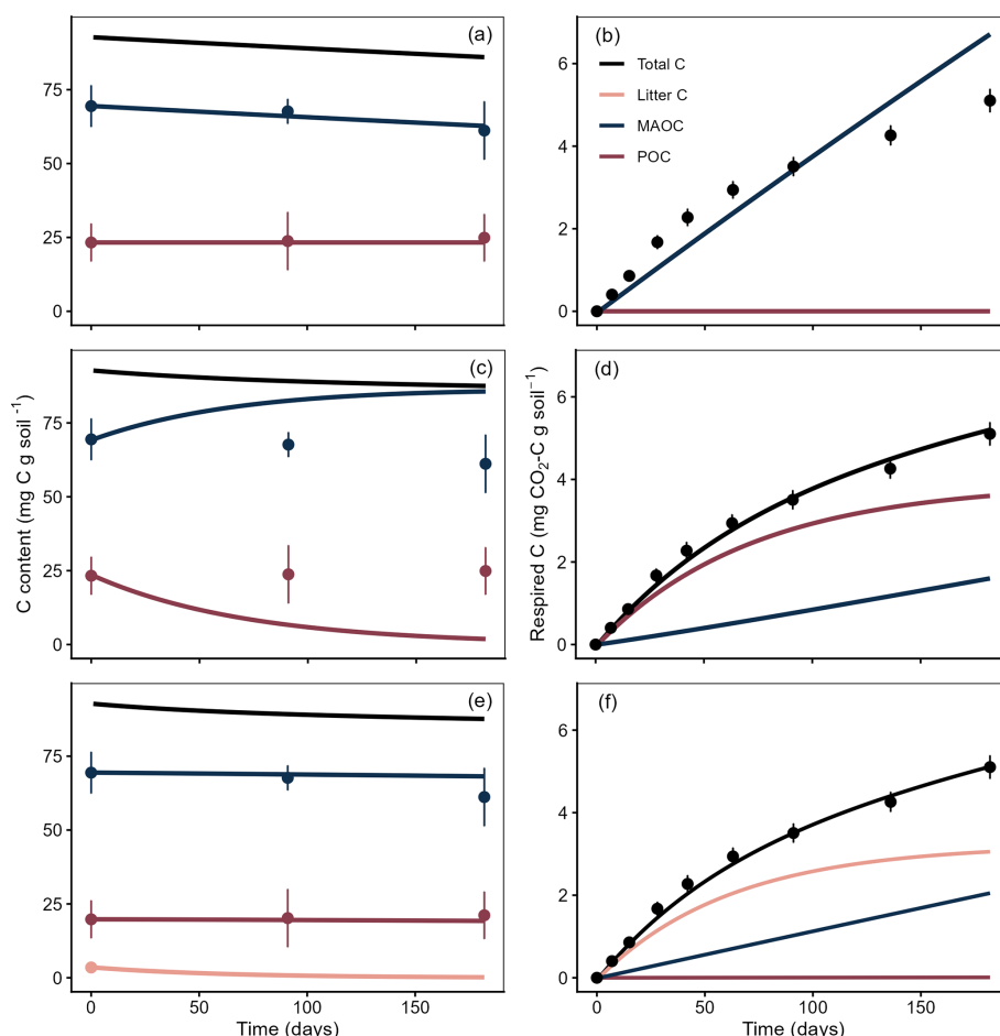
Figure 2. C content (a, c, e) and respired C (b, d, f) in each C pool and total in control soils (no litter-addition). In black, Total C; in dark blue, MAOC; in dark red, POC; in pink, Litter C. The lines represent the model estimations, while the points represent the observed data. (a, b) 2-pool models that best fitted C pools content. (c, d) 2-pool models that best fitted the respiration. (e, f) 3-pool model.
