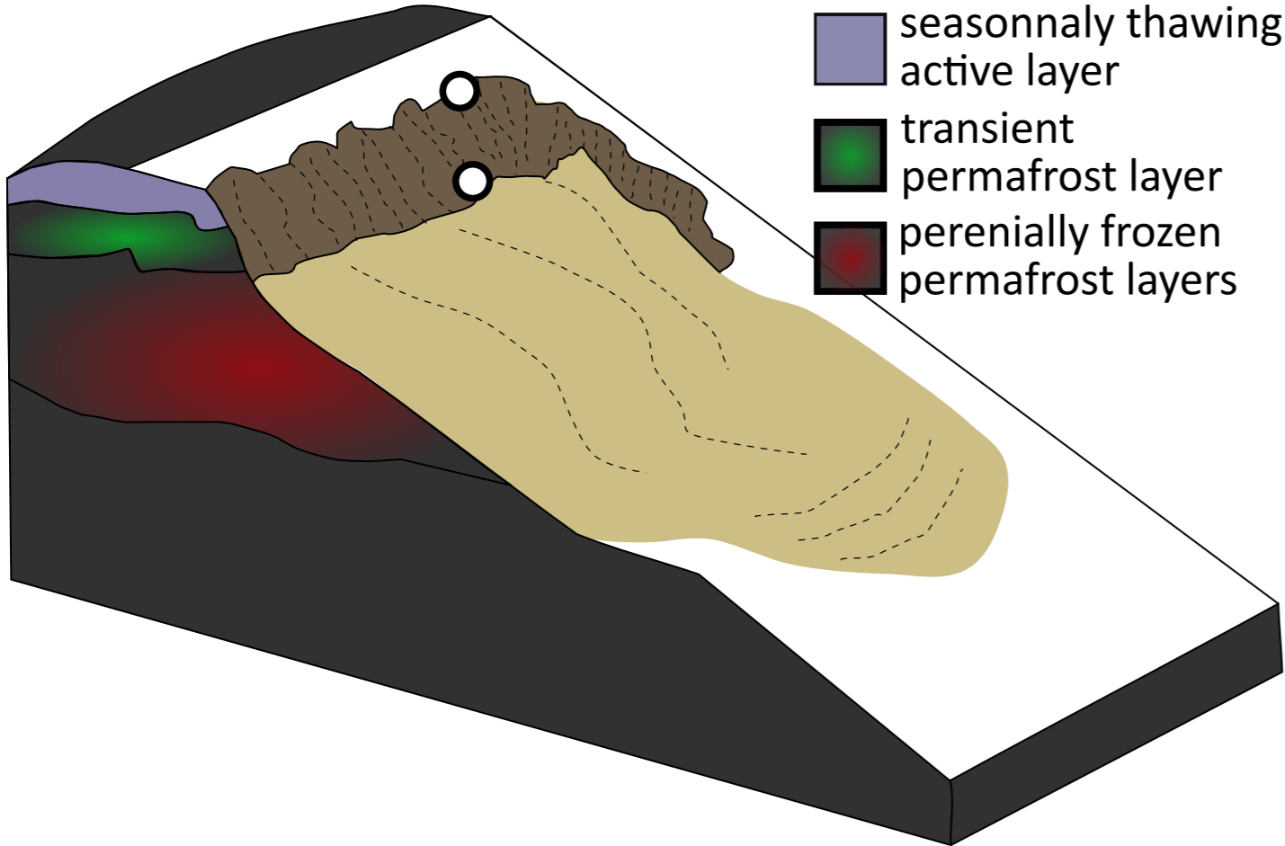
a Retrogressive thaw slump
