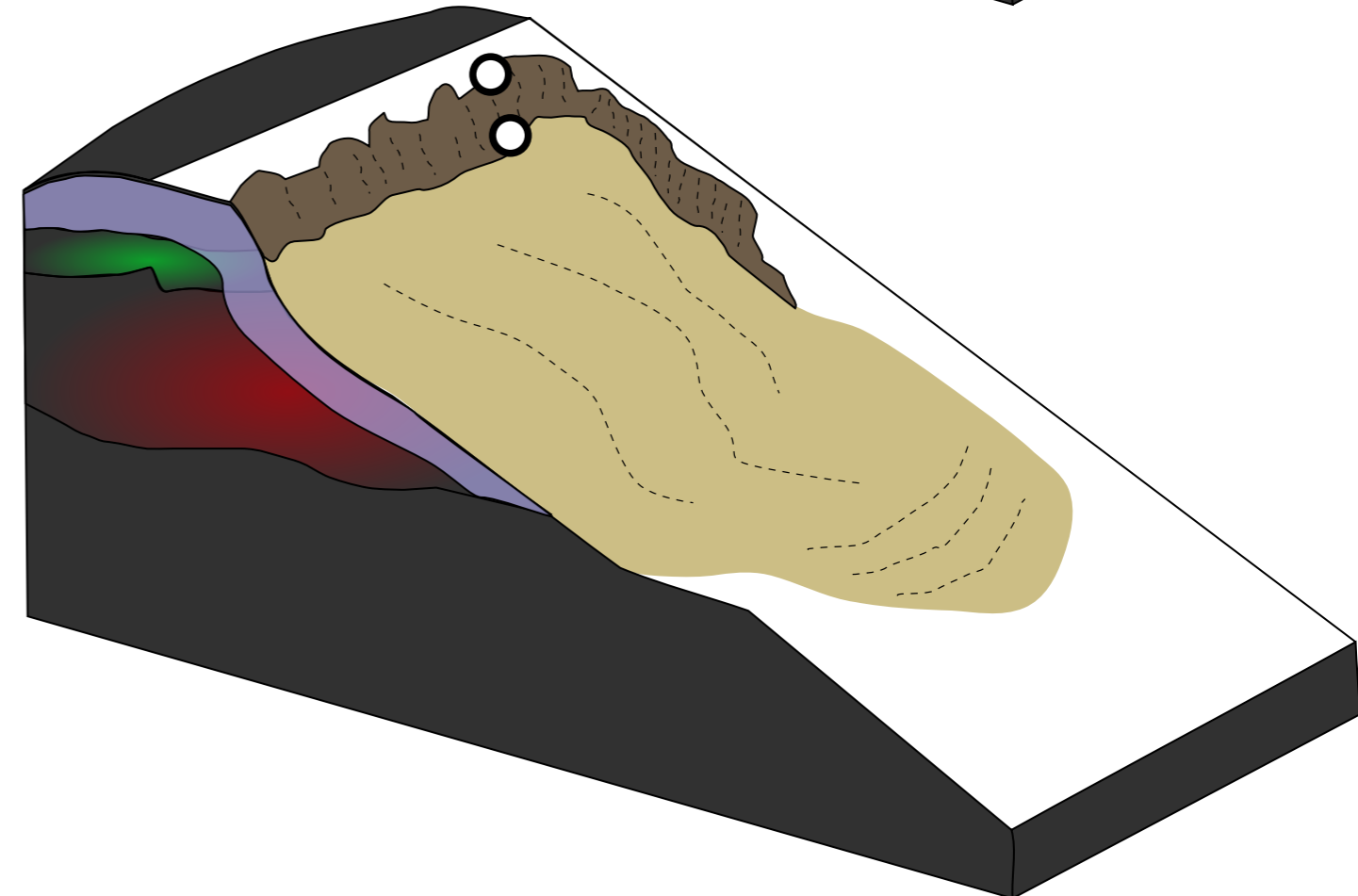
c 'old' active layer detachment
