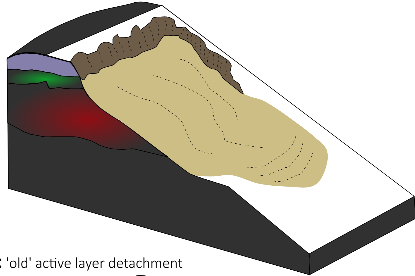
b 'fresh' active layer detachment
