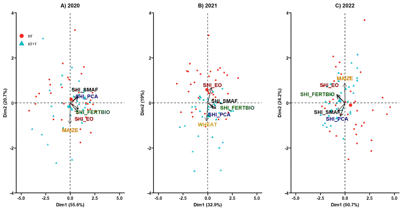
Figure 6. Principal component analysis (PCA) of soil health indices (SHI_PCA, SHI_EO, SHI_FERTBIO, and SHI_SMAF) and crop yield under no-till (NT) and no-till with terraces (NT + T) for the years 2020 (a), 2021 (b), and 2022 (c). In 2022, NT + T enhanced soil health indices and strengthened their association with crop productivity under the evaluated field conditions. Differences were statistically significant ( p < 0.05 ; 999 permutations).
