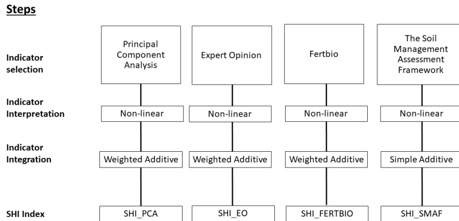
Figure 2. Steps followed to generate soil health indices: SHI_PCA, SHI_EO, SHI_FERTBIO and SHI_SMAF.
