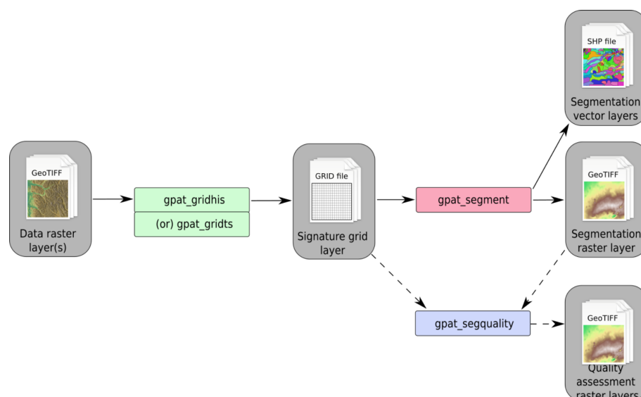
Figure 3.13: Workflow path for segmentation
