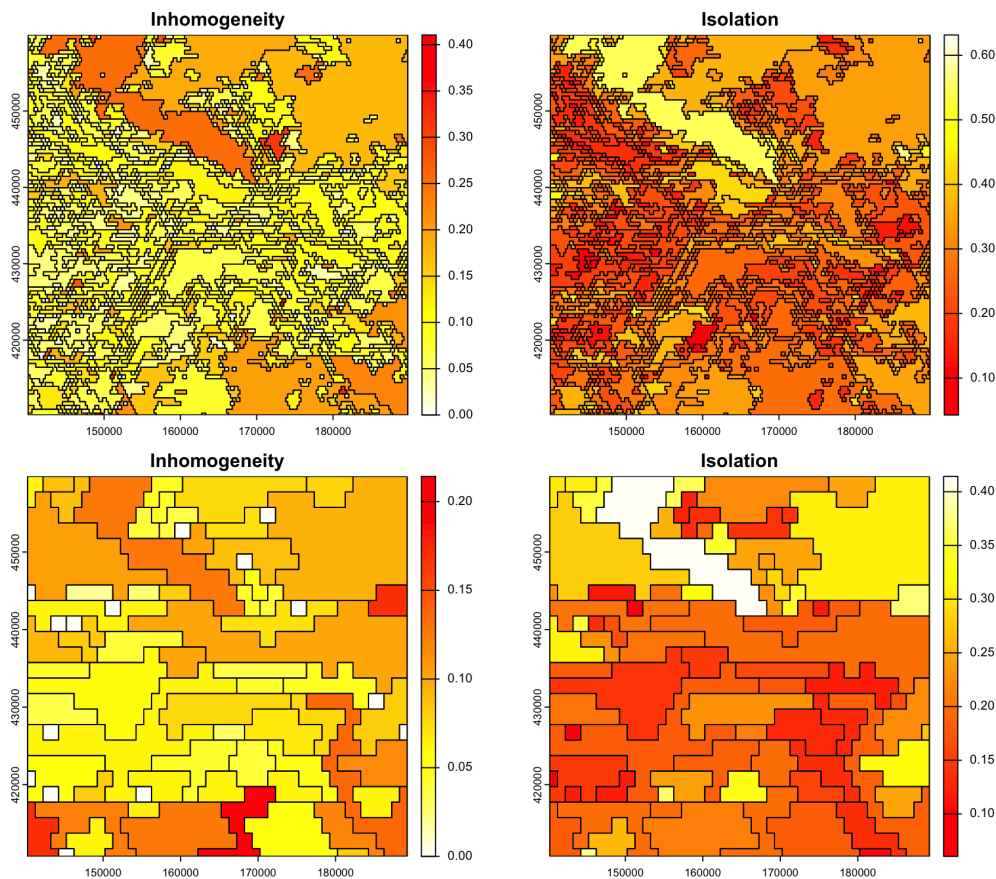
Figure 9. Evaluation of segmentation based on bulk density over the whole profile at the 1 : 100 000 (top) and 1 : 400 000 (bottom) design scales. Note the different colour ramps for the two scales.
