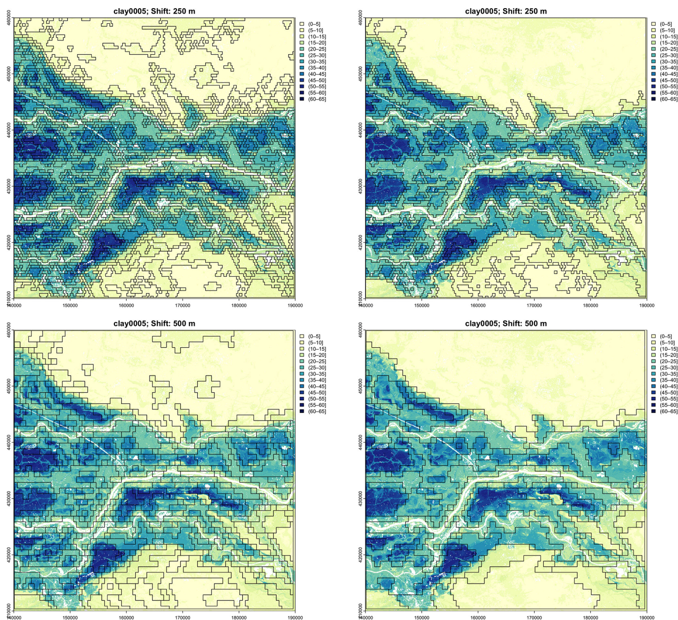
Figure 12. Segmentation by whole-profile clay at 1 : 100 000 (top) and 1 : 200 000 (bottom) with default thresholds (left) and liberal thresholds (right), overlaid on the clay 0–5 cm DSM product.
