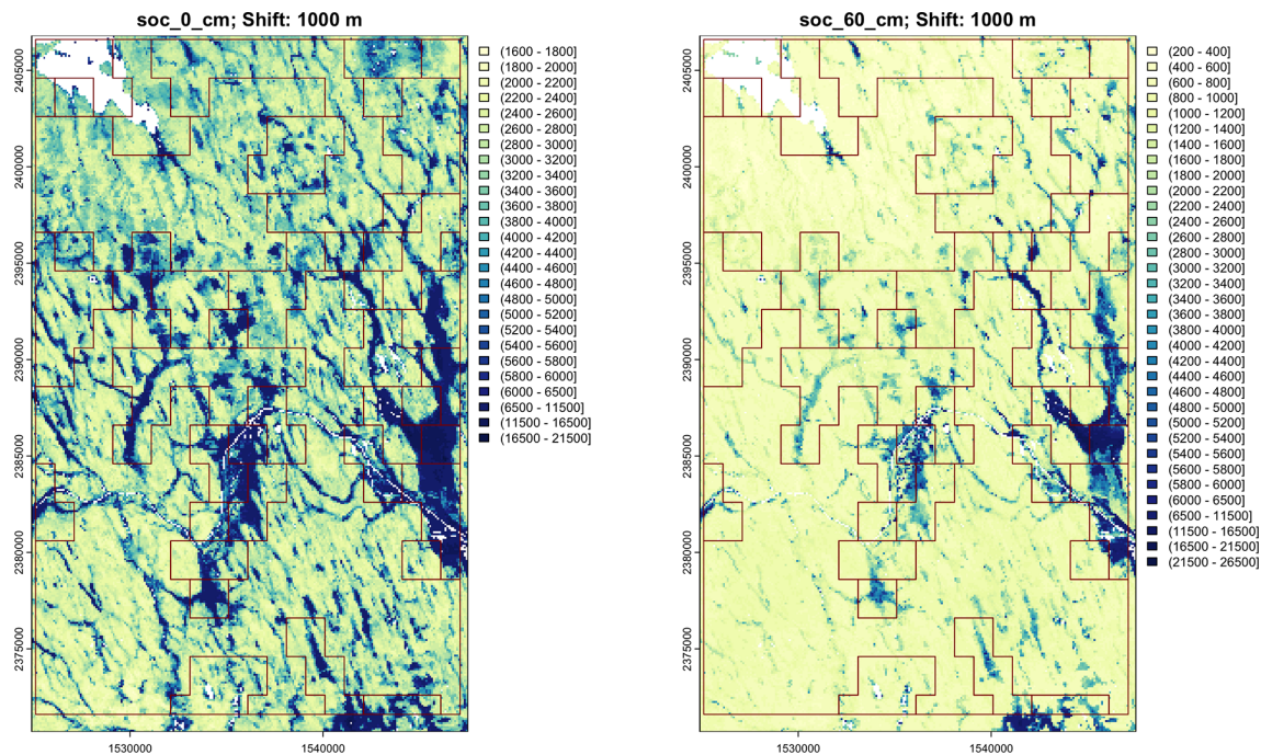
Figure 28. Segmentation based on all depth slices of SOLUS-predicted SOC concentration, nominal scale 1 : 400 000, 1000× %. Note the slightly different colour scales.
