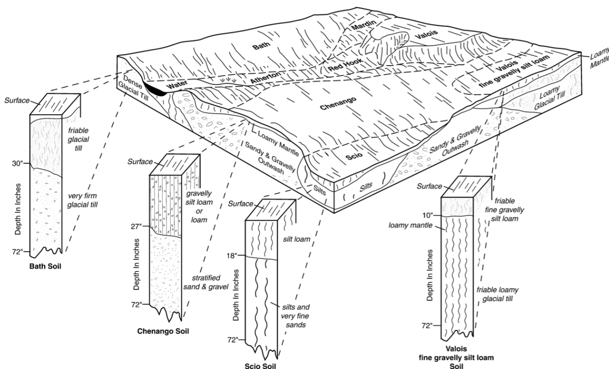
Figure 1. Conceptual block diagram, Otsego County NY (USA). Source: https://www.nrcs.usda.gov/publications/NY-2010-09-28-14.png (last access: 9 October 2025).
