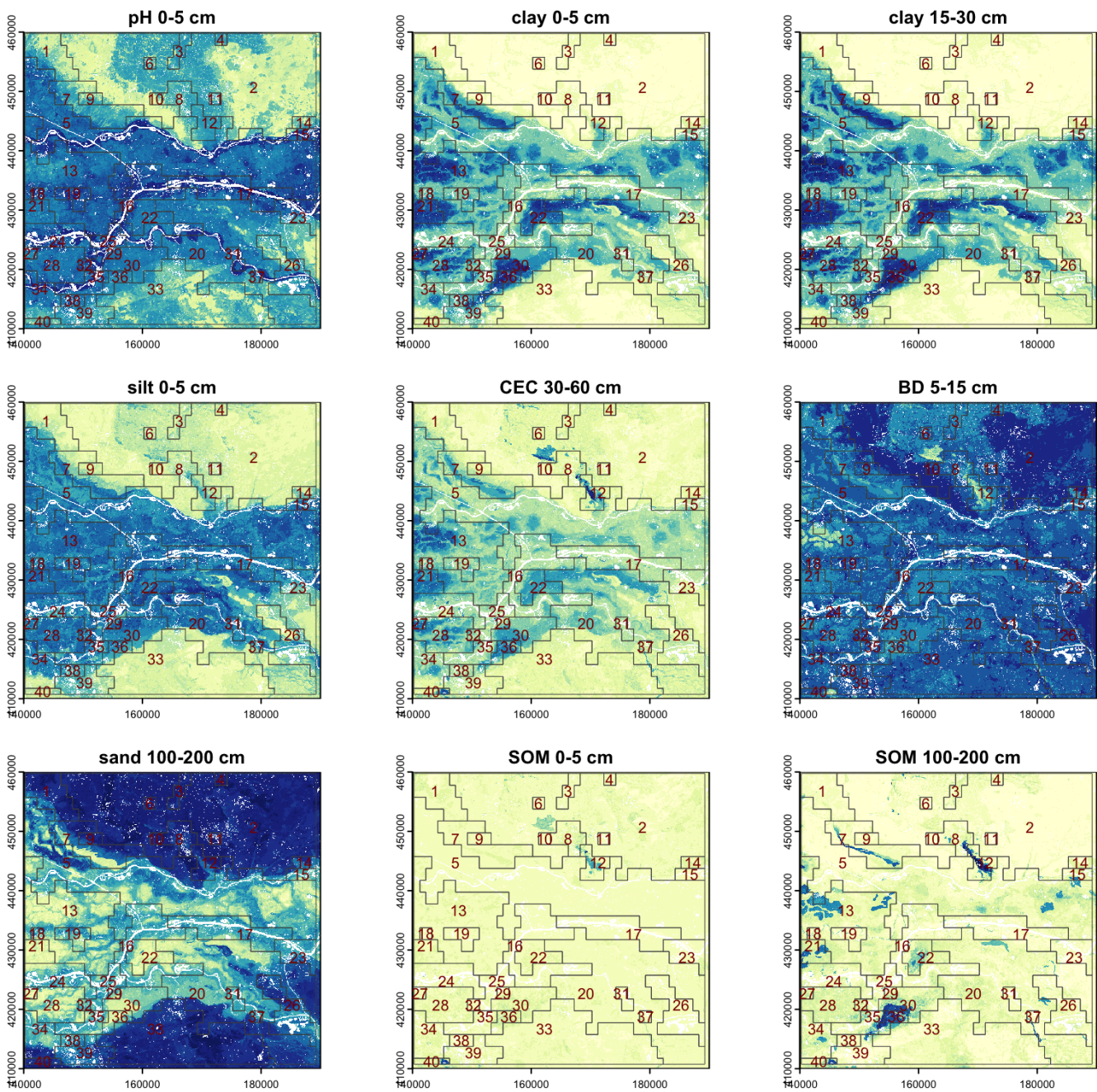
Figure 10. Segmentation based on selected properties and depth slices, overlaid on DSM of selected soil properties, 1 : 400 000 design scale. Legends not shown. Scale is from yellow (low values of the property) to dark blue (high values). Segments are labelled with their numbers.
