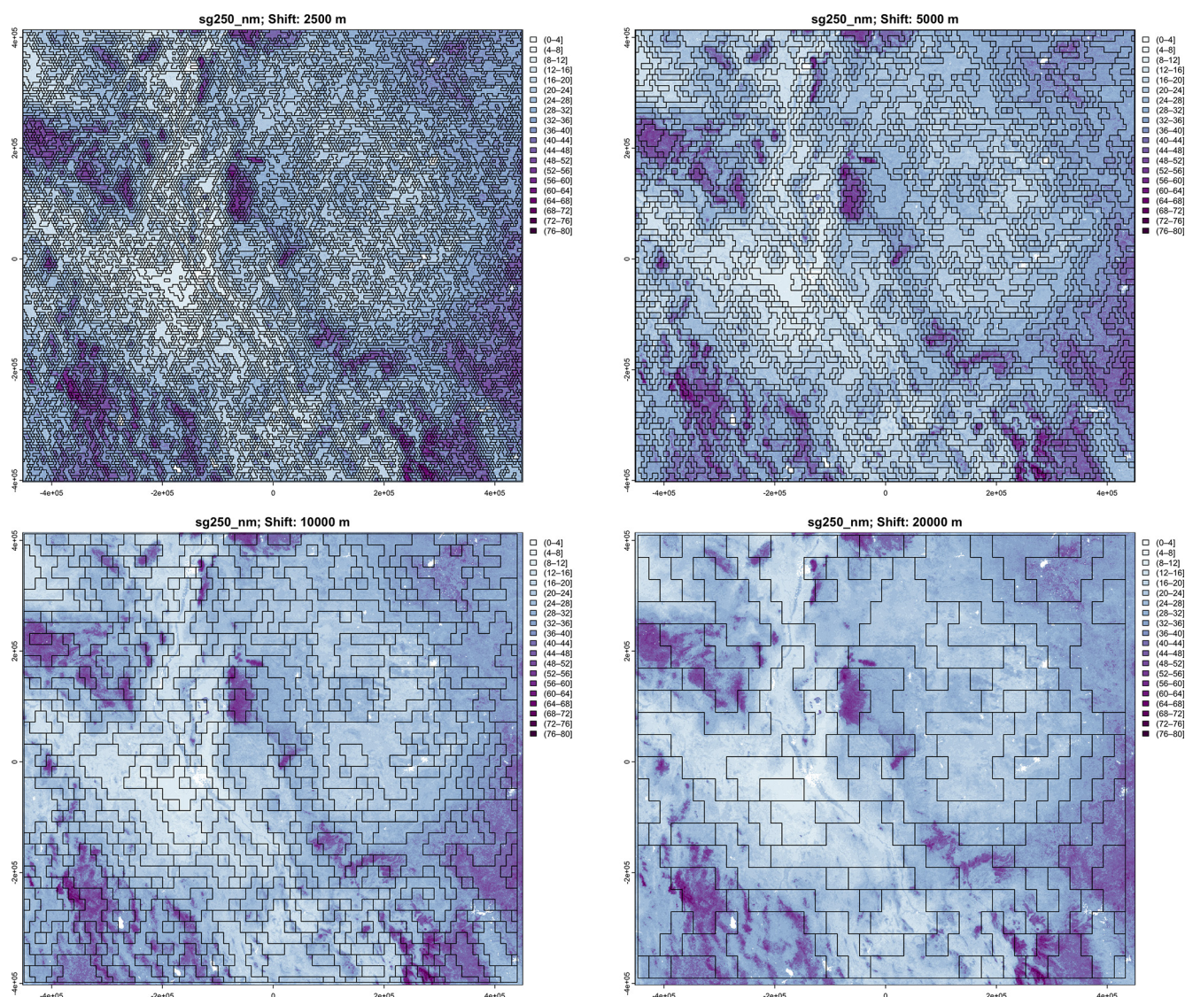
Figure 19. Segmentation of the SoilGrids v2.0 250 m resolution SOC stock map (part) at (left to right, top to bottom) 1 : 1 000 000, 1 : 2 000 000, 1 : 4 000 000 and 1 : 8 000 000 nominal resolutions. Units are \text{T ha}^{-1} .
