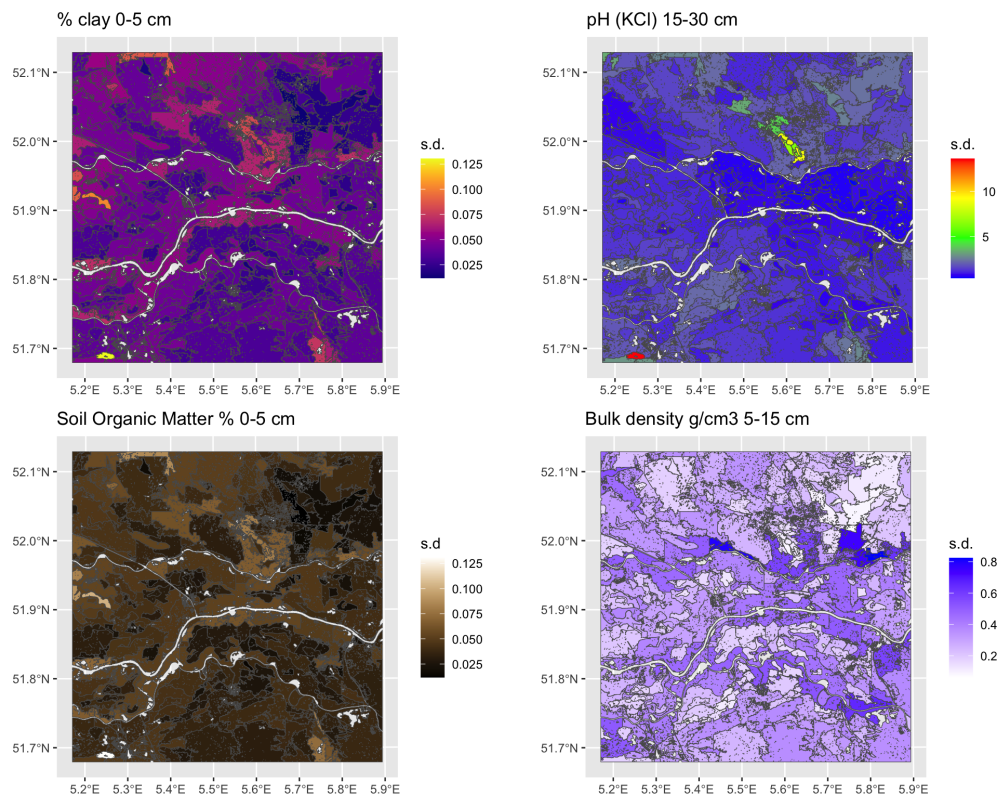
Figure 6. Standard deviations for selected properties of aggregation by supercells algorithm using all properties and layers.
