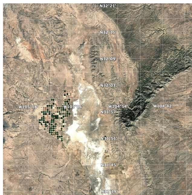
Figure 16. Test area for aggregation, centred on (-105^\circ \text{E}, 32^\circ \text{N}) . Source: © Google Earth.
