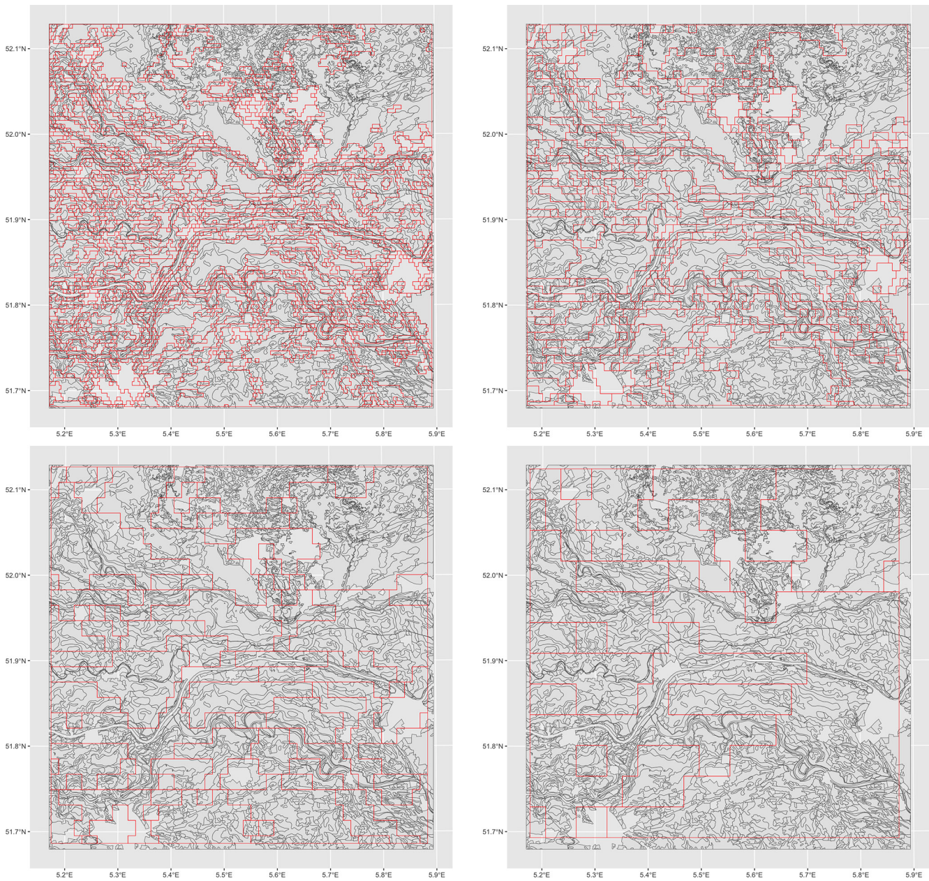
Figure 8. Segmentation based on bulk density over the whole profile (red lines), overlaid on soil map polygons (grey lines). Design scales left to right, top to bottom: 1 : 100 000, 1 : 400 000, 1 : 800 000, 1 : 1 600 000.
