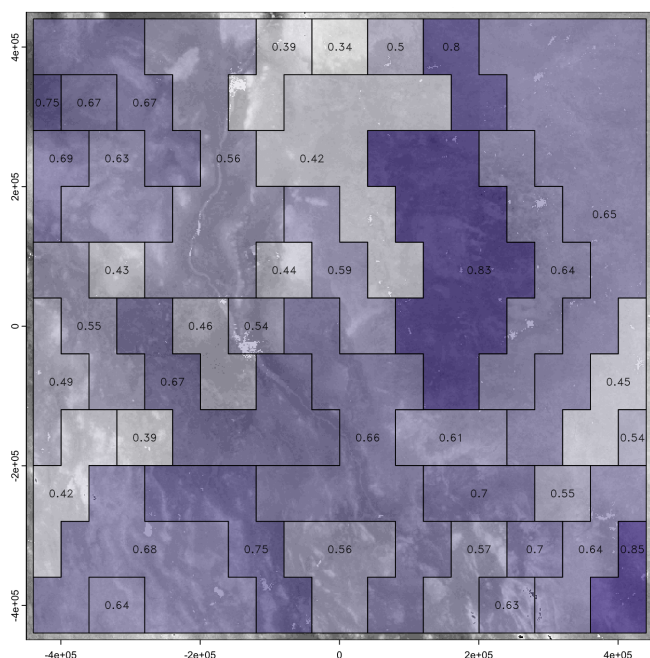
Figure 21. Normalized Shannon Entropy of segments of the v2.0 1 km resolution SOC stock map (part) at 1 : 16 000 000 nominal resolution. Colour scale from white (lowest entropy) to dark purples (highest entropy).
