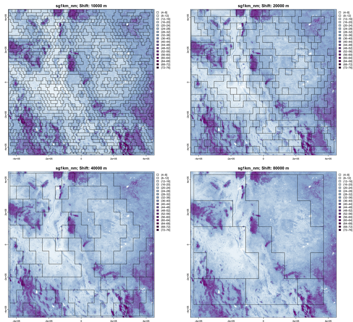
Figure 20. Segmentation of the SoilGrids v2.0 1 km resolution SOC stock map (part) at (left to right, top to bottom) 1 : 2 000 000, 1 : 4 000 000, 1 : 8 000 000, and 1 : 16 000 000 nominal resolutions. Units are \text{T ha}^{-1} .
