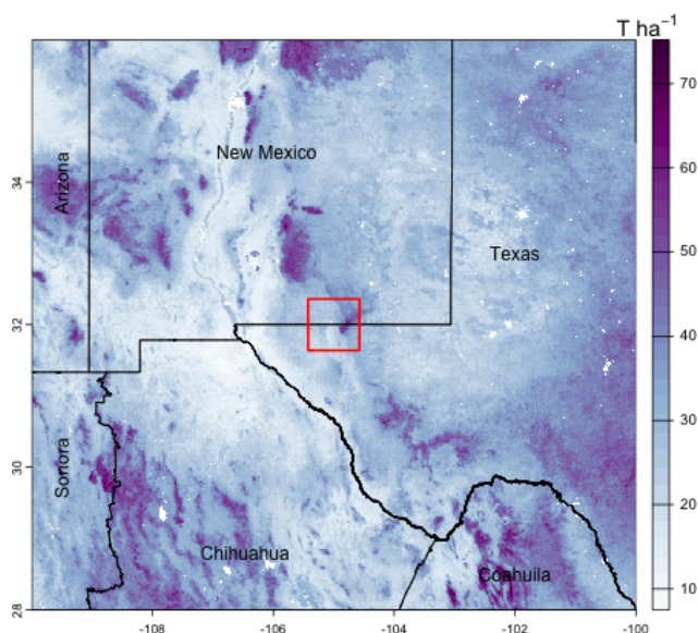
Figure 15. SoilGrids v2.0; SOC stock 0–30 cm, \text{T ha}^{-1} . Test area for aggregation (Sect. 4.1) shown as a red square.
