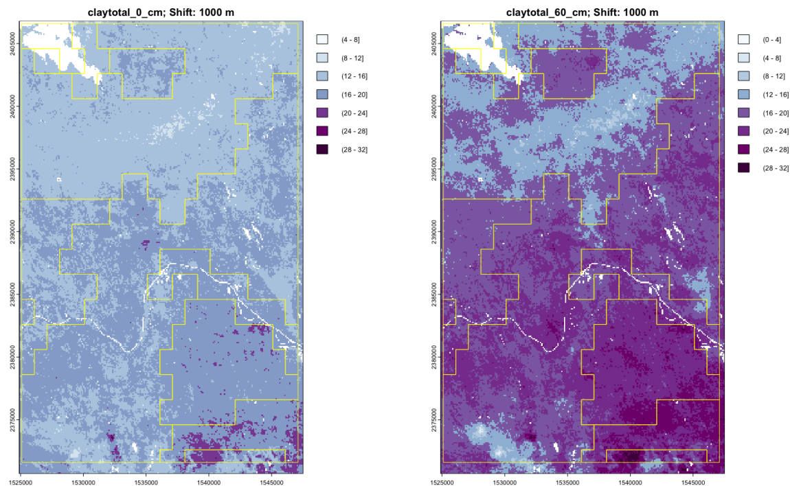
Figure 29. Segmentation based on all depth slices of clay concentration, nominal scale 1 : 400 000, %. Note the slightly different colour scales.
