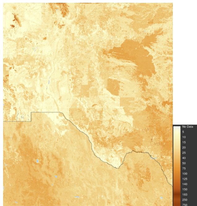
Figure 30. Global Soil Organic Carbon (GSOC) map (part). Boundary is between México (south) and the USA (north). Values are \text{T ha}^{-1} SOC stock. Source and legend: FAO (2024).
