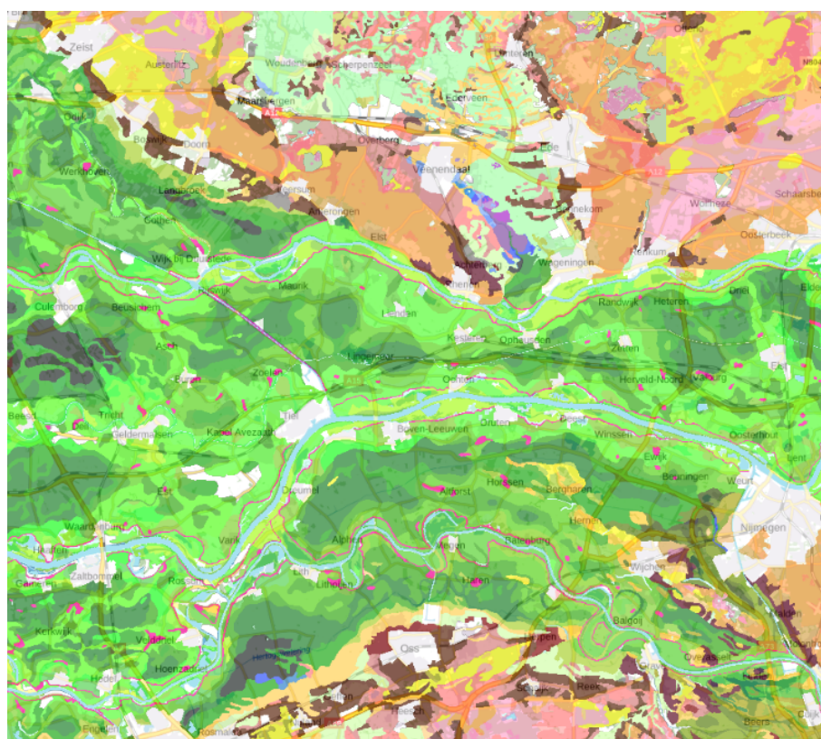
Figure 4. Semi-detailed soil map of the Netherlands, design scale 1 : 50 000 (part). Source and detailed legend: Ministerie van Volkshuisvesting en Ruimtelijke Ordening (2024). General legend: Dark and medium green: river clays with different clay concentrations; Light green: glacial depression sediments; Brown, pink: push moraines with varying sand and gravel sizes; Yellow: wind-blown sands; Purple: peat.
