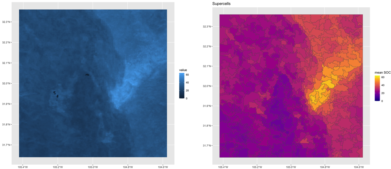
Figure 17. SoilGrids v2.0 250 m SOC stock 0–30 cm, T ha −1 (left) and its aggregation into supercells (right).
