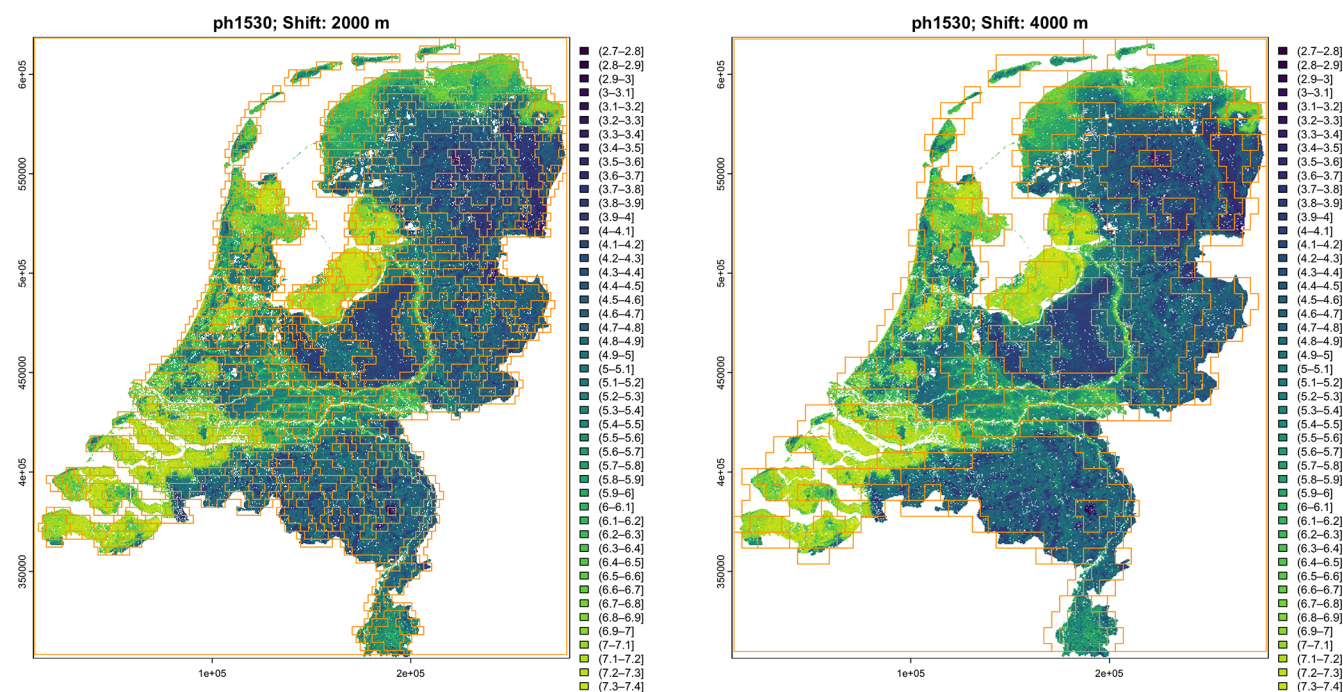
Figure 11. Segmentation by whole-profile pH of the Netherlands at 1 : 800 000 (left) and 1 : 1 600 000 (right) nominal scales, overlaid on the pH 15–30 cm DSM product.
