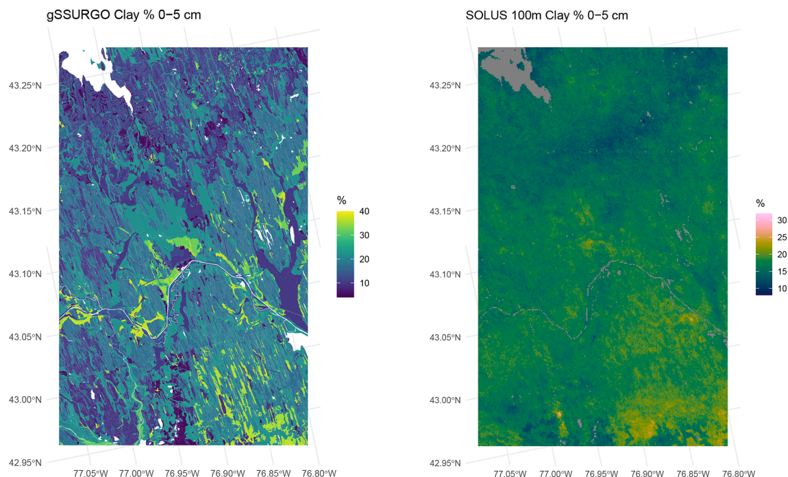
Figure 26. Clay concentration % of the 0–5 cm layer, gSSURGO (left), SOLUS 100 m (right).
