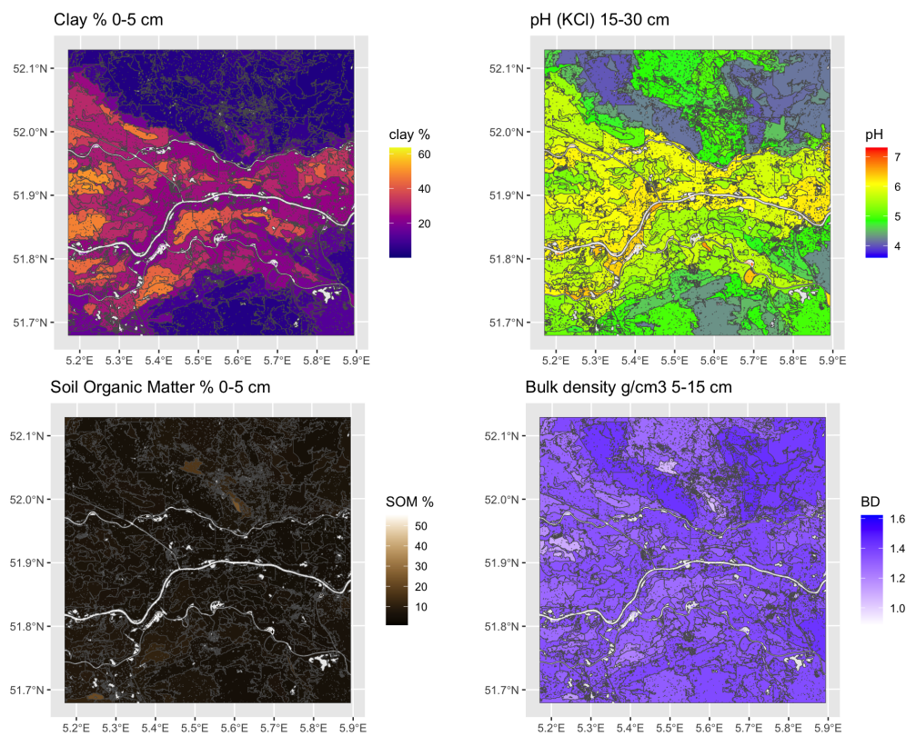
Figure 5. Results for selected properties of aggregation by supercells algorithm using all properties and layers.
