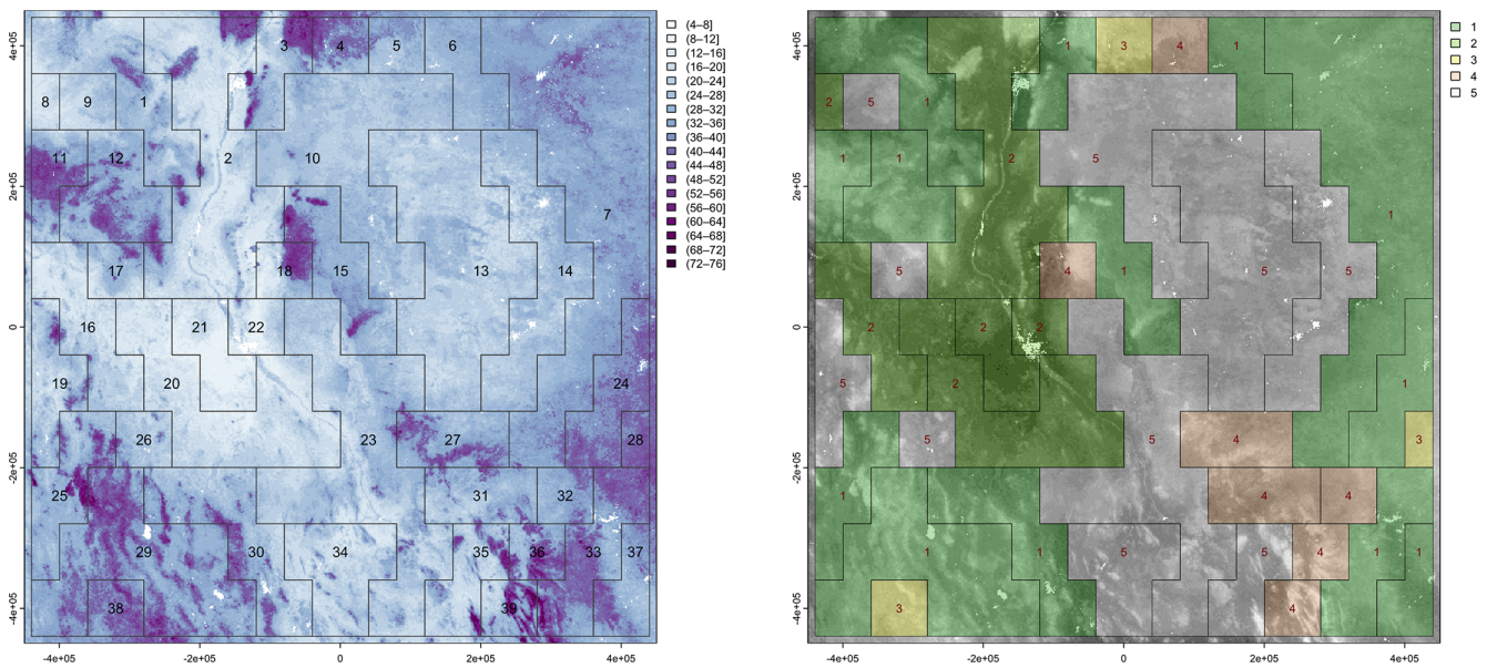
Figure 22. (left) Segmentation of the SoilGrids v2.0 1 km resolution SOC stock map, motif size 40 cells, units are \text{T ha}^{-1} ; (right) assignment of segments to five generalised clusters, legend is cluster number.
