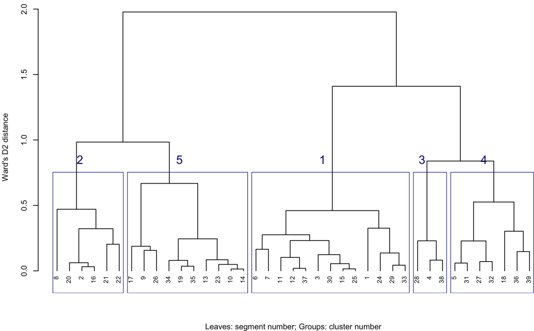
Figure 23. Dendrogram of segment signatures, SoilGrids v2.0 1 km SOC stock map, motif size 40 cells, with five general clusters.
