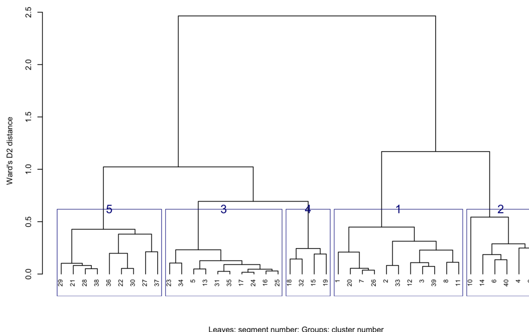
Figure 13. Hierarchical clustering of the segments shown in Fig. 10.
