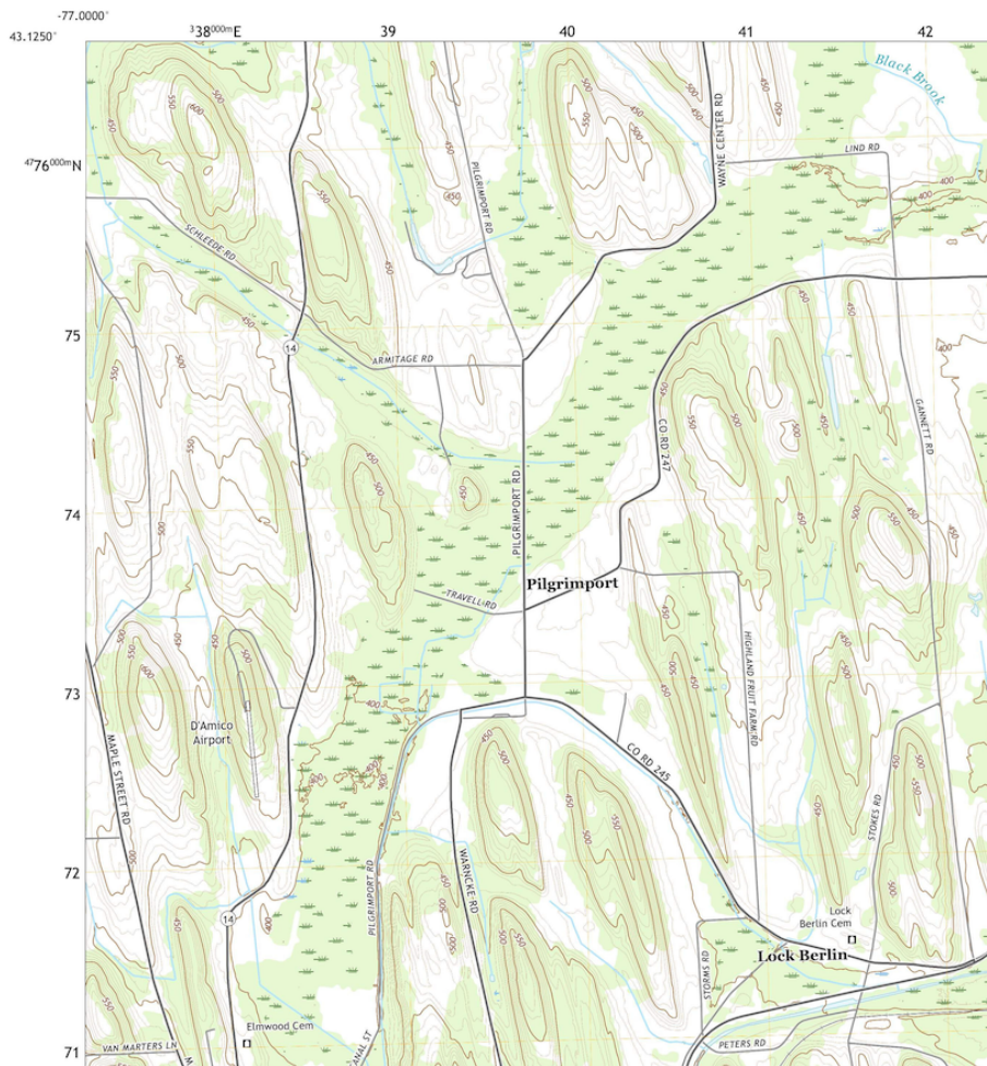
Figure 25. Representative portion of the SOLUS100 test area. Source: USGS topographic map, Lyons NY quadrangle, 2016, scale 1 : 24 000. Contour interval 10 ft. (approx. 3.048 m). Projection and marginal coordinates UTM Zone 18N. The centre swamp contains Typic Medisaprists; drumlin tops are Glossic Hapludalfs.
