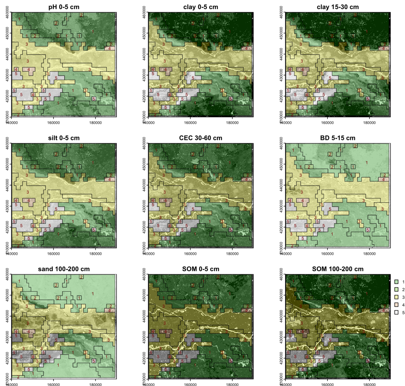
Figure 14. Generalised clusters of the segmentation of Fig. 10, based on slicing the clustering dendrogram shown in Fig. 13. The same segmentation is shown for nine selected property-depth combinations. Clusters shown by colour and number.
