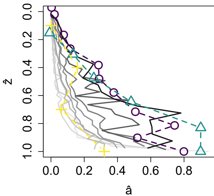
(c) Bioturbated fraction
