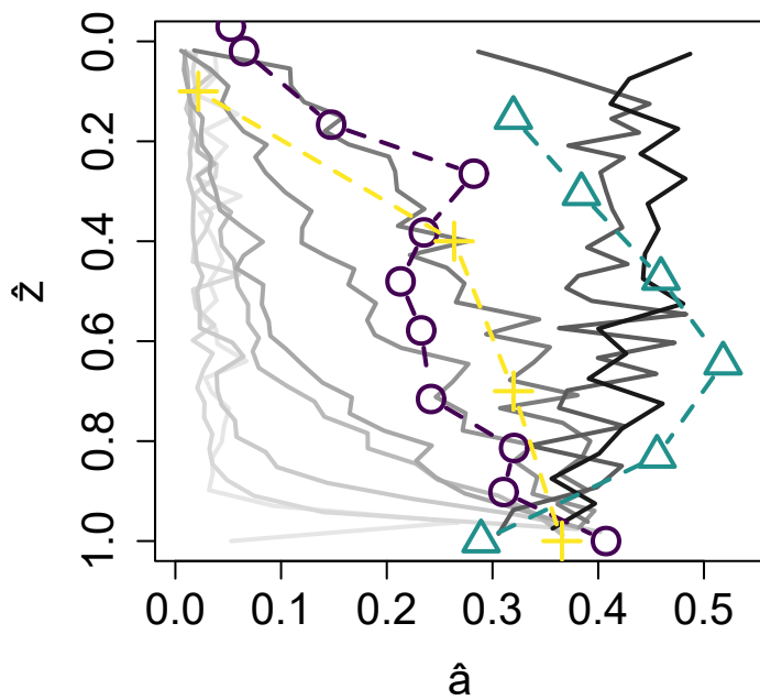
(b) Interquartile range
