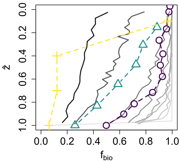
(c) Bioturbated fraction
