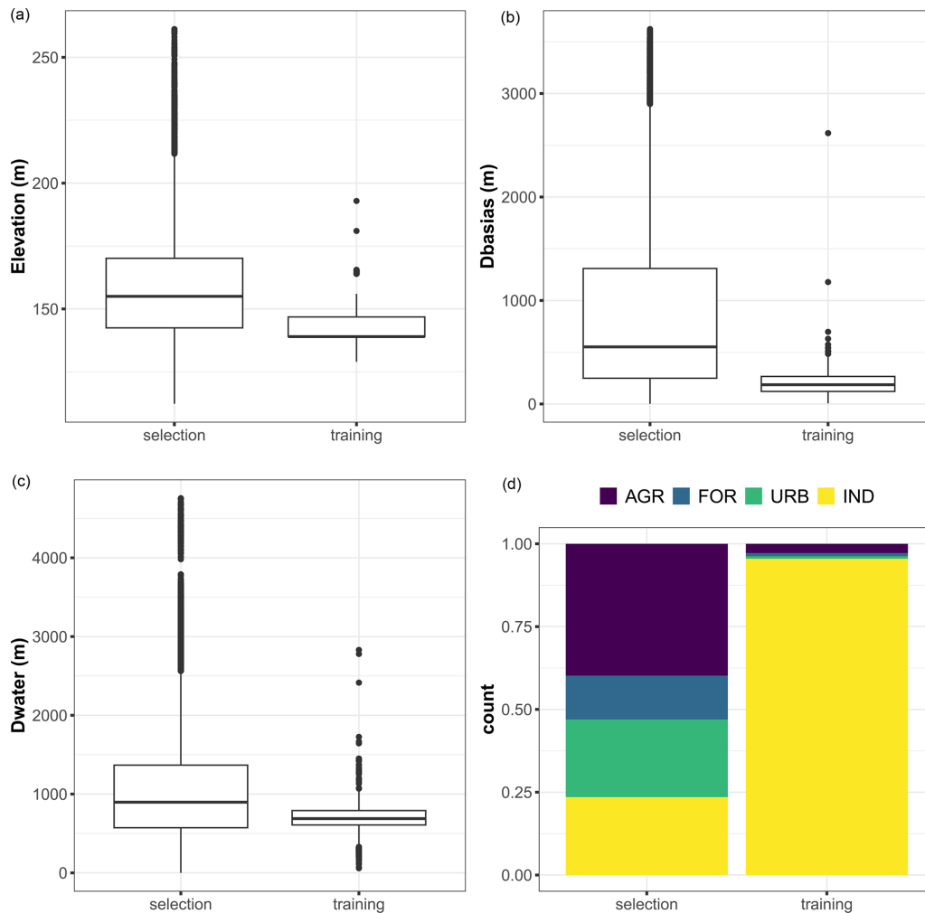
Figure 12. Boxplots of the covariate values for the training dataset and for the locations (named selection) where the corresponding group of covariates significantly contributes to the best estimate, with a scaled Shapley value exceeding that of the uncertainty by more than 25 %. Panel (d) compares the proportions of land use categories (AGR: agriculture, FOR: forests and grasslands, and IND: industrial and commercial economic activities) for the selection and training datasets.
