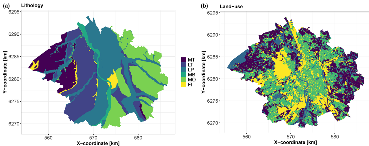
Figure 5. Covariates of categorical type over the city of Toulouse. (a) Lithology (MT: medium terrace alluviums, LT: low terrace alluviums, LP: low plain alluviums, MB: major riverbed alluviums, MO: molasses, and FI: fill materials). (b) Land use (AGR: agriculture, FOR: forests and grasslands, and IND: industrial and commercial economic activities); see Table 2 for a detailed description.
