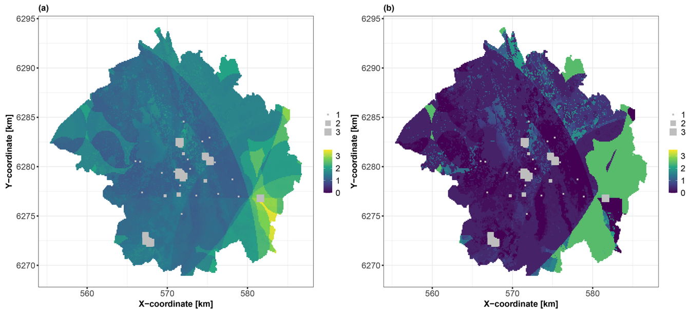
Figure 9. (a) Prediction best estimate of the hydrocarbon concentration ( \log_{10} scale) for the city of Toulouse using the conditional mean of the RF model. The soil samples are indicated by squares whose sizes are proportional to the \log_{10} of the hydrocarbon concentration. (b) Interquartile width (IQW) computed using the 25th and 75th percentiles of the qRF model (expressed on the same scale as the hydrocarbon concentration).
