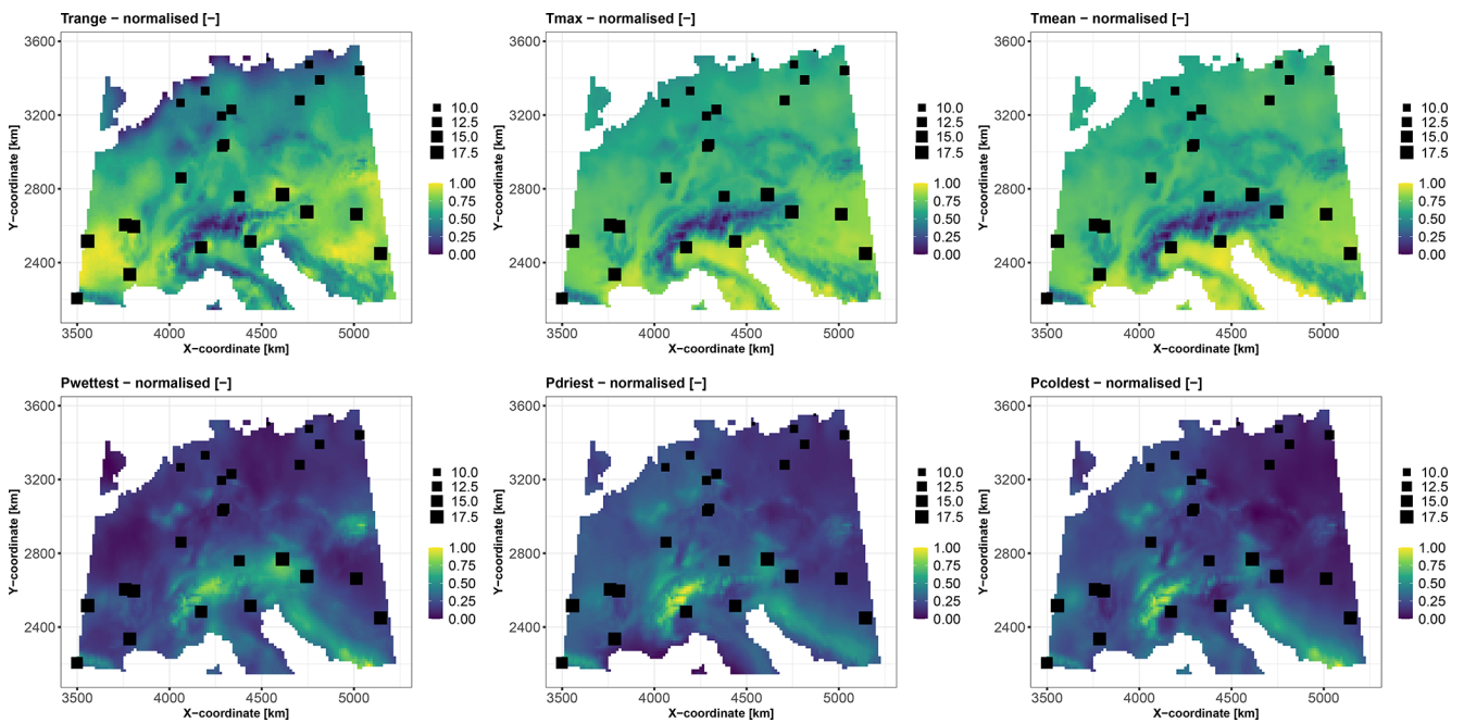
Figure 2. Covariates (with prior normalisation between 0 and 1) used in the synthetic test case (see Table 1 for a detailed description). The spatial distributions of the 25 soil samples are indicated by square-shaped markers. The size of each square is proportional to the synthetic variable calculated from the covariates based on Eq. (1).
