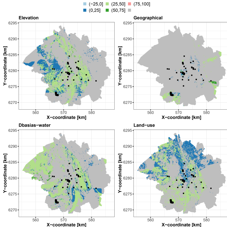
Figure 11. Locations where each corresponding group of covariates significantly contributes to the best estimate, with a scaled Shapley value exceeding that of the uncertainty by more than 25 %. The colours indicate the scaled Shapley value for the best estimate. The areas in grey correspond to grid points where the condition is not met. The black squares indicate the locations of the soil samples used for RF training.
