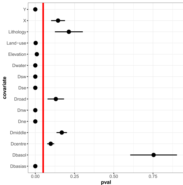
Figure 8. Screening analysis showing the p values (denoted pval) of the HSIC-based test of independence (described in Appendix C) for the Toulouse case. The dots indicate the mean values estimated over the replicates of a 10-fold cross-validation (repeated 25 times). The lower and upper bounds of the error bars are defined as \pm 1 standard deviation. When the dot merges with the error bar, the value of the standard deviation is low. The vertical red line indicates the significance threshold at 5%. When the p value is lower than 5%, the null hypothesis should be rejected; i.e. the considered covariate has a significant influence on the hydrocarbon concentration and is retained in the RF construction.
