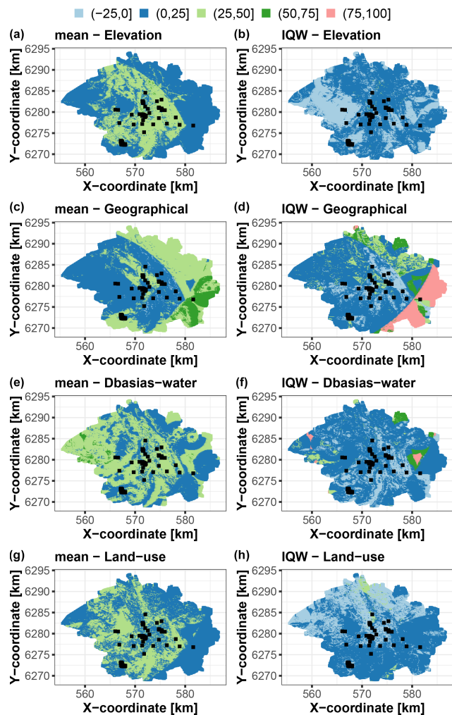
Figure 10. Scaled Shapley values (in %) for each group of covariates of the Toulouse test case considering the prediction best estimate using the RF conditional mean ( a , c , e , g ) and the prediction uncertainty using the qRF interquartile width (IQW) ( b , d , f , h ). The black squares indicate the locations of the soil samples used for RF training.
