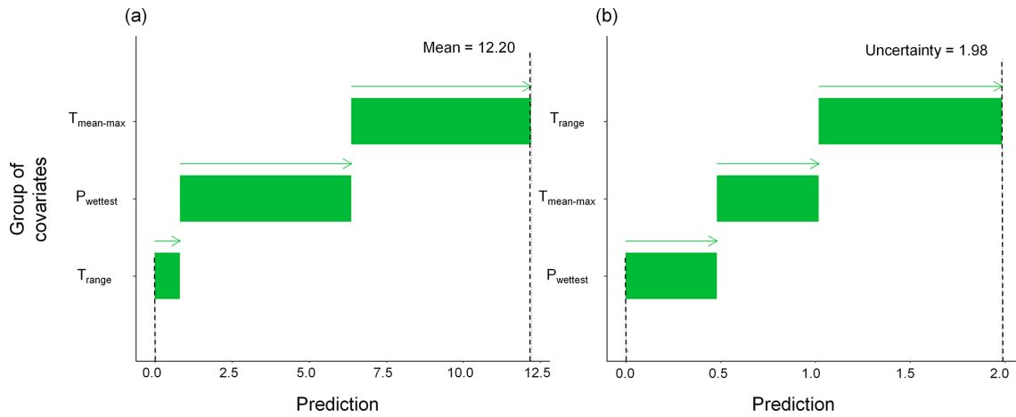
Figure 1. Example of SHAP-based decomposition of the prediction best estimate (modelled by the conditional mean of a random forest model; panel a ) and of the prediction uncertainty (modelled by the interquartile width estimated via a quantile random forest model; panel b ) for the variable of interest in the synthetic test case (fully described in Sect. 2.1) at a certain location in the study area. Each horizontal bar represents the contribution to the prediction (indicated by the vertical dashed line) of the considered covariates (indicated on the vertical axis) that correspond to the mean diurnal range, T_{range} , to the group of covariates that includes the maximum and mean temperatures of the warmest quarter of the year, T_{mean-max} , and to the precipitation of the wettest month, P_{wettest} . Note the differences in the ordering of the groups, which indicates that the contributors to the mean and to the uncertainty estimate differ.
