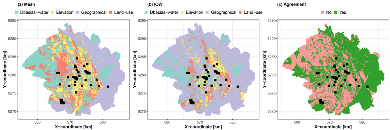
Figure 13. Spatial distributions of the most important group of covariates with respect to the scaled Shapley values for the prediction best estimate (mean; panel a) and for the prediction uncertainty (IQW; panel b) in the city of Toulouse. Panel (c) shows the regions where the most important group of covariates for the mean agrees with that for IQW. The black squares indicate the locations of the soil samples used for RF training.
