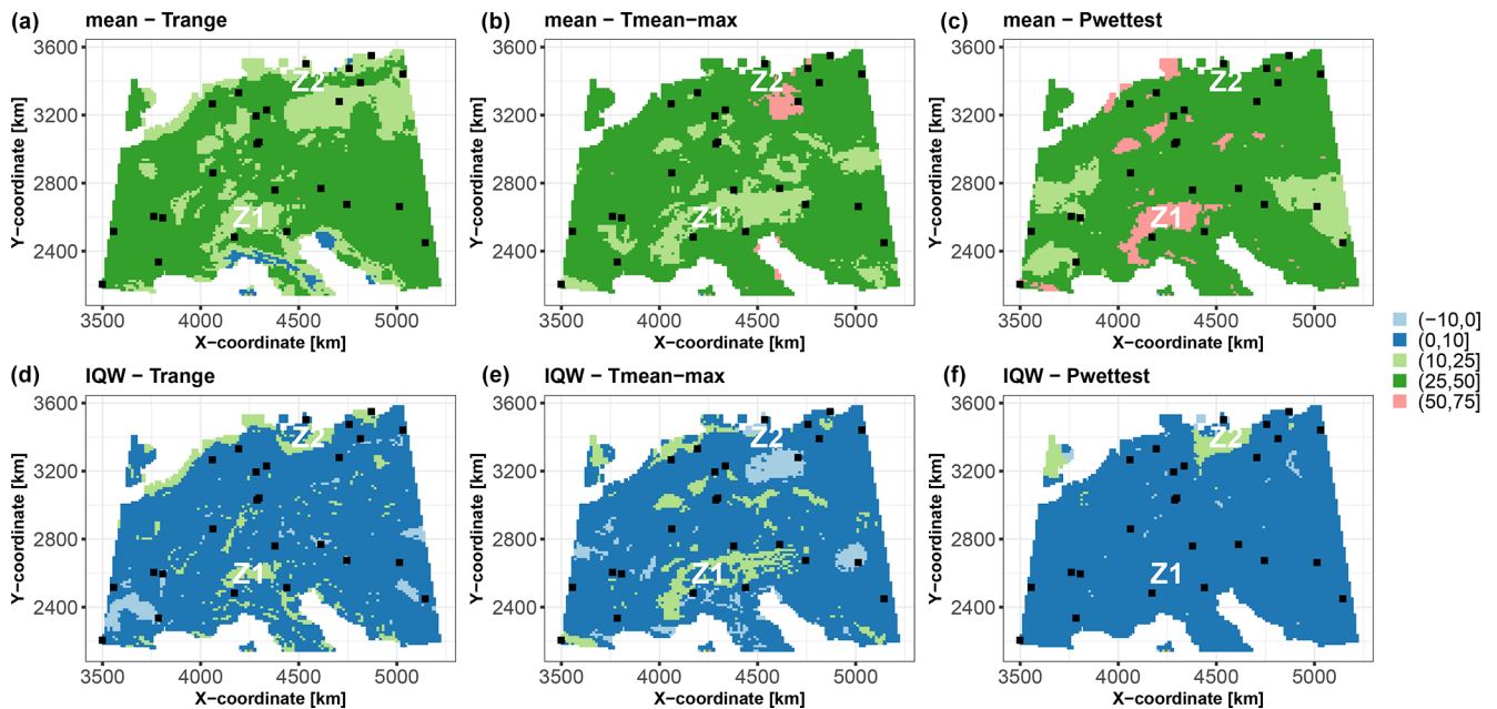
Figure 7. Scaled Shapley values (in %) for the synthetic test case considering the prediction best estimate modelled by the RF conditional mean (a–c) and the prediction uncertainty modelled by the qRF interquartile width (IQW; d–f). The black squares indicate the spatial locations of the 25 soil samples. The results are more specifically discussed in Sect. 4.1 for the zones indicated by Z_1 and Z_2 .
