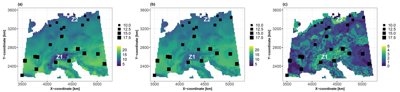
Figure 6. (a) Spatial distribution of the synthetic variable of interest modelled by Eq. (1). (b) Prediction best estimate using the conditional mean of the RF model. (c) Interquartile width (IQW) computed using the 25th and 75th percentiles of the qRF model. The 25 soil samples are indicated by squares whose sizes are proportional to the value of the synthetic variable of interest. The results are more specifically discussed in Sect. 4.1 for the zones indicated by Z_1 and Z_2 .
