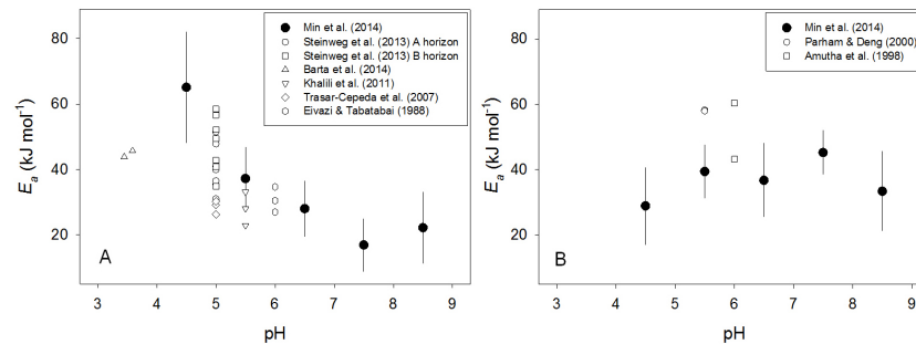
Figure 1. Estimates of intrinsic (closed symbols) and apparent (open symbols) E_a for the BGase/BG reaction (a) and the NAGase/NAG reaction (b). The literature values for apparent E_a are shown at the pH at which the reaction was actually observed, and does not necessarily correspond to the pH of the soils from which the samples were taken. See Sect. 3 for interpretation.
